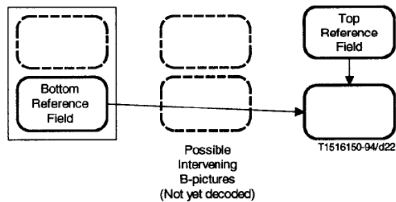
Figure 7-7 – Prediction of the second field-picture when it is the bottom field
