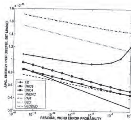
Figure 6.7. Energy efficiency of coding schemes for point-to-point links. Wire lengths are in the order of millimeters.
