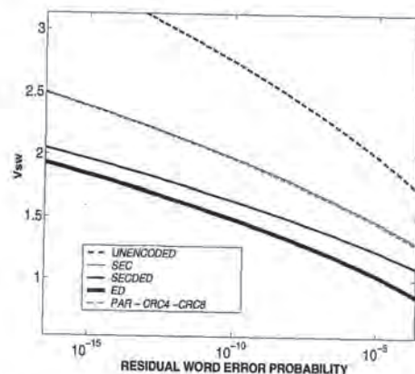
Figure 6.5. Minimum voltage swing needed by each coding scheme to meet a predefined communication reliability requirement.
