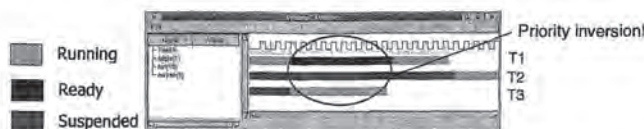
Figure 13 Detection of priority inversion by OS architecture level simulation.
