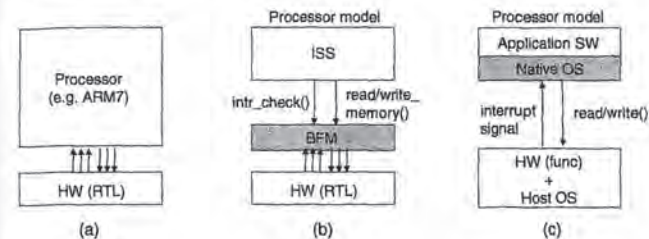
Figure 5 Conventional methods of validating OS implementations.
