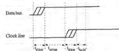
Figure 8.1. Latest allowed safe arrival for data signals w.r.t the clock.
