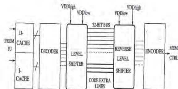
Figure 6.4. Realistic SoC setting where the energy-reliability trade-off is investigated.
