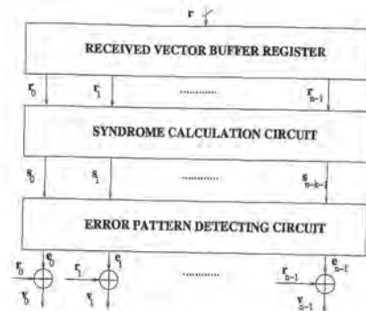
Figure 6.1. Decoder for a Hamming code.
