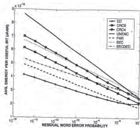
Figure 6.6. Energy efficiency of coding schemes for point-to-point links. Wire lengths are in the order of centimeters.
