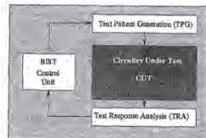
Figure 4. A generic architecture of BIST
