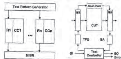
Figure 8. BIST architectures
