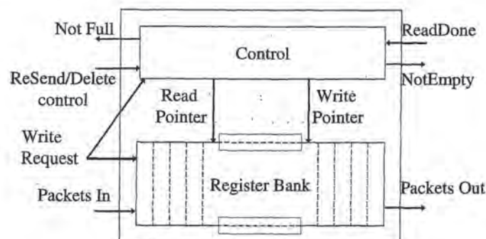
Figure 10.9. Structure of Proteo FIFO.
