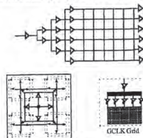
Figure 8.5. Common buffered trees. a) Tapered H-tree. b) Mesh
