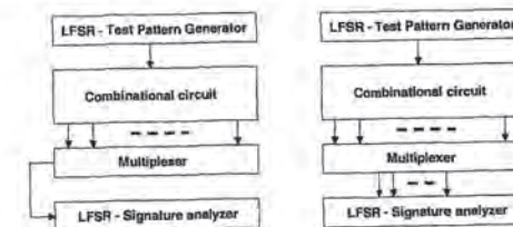
Figure 6. Single input and multiple input signature registers
