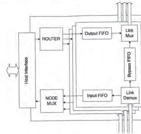
Figure 10.6. Advanced node architecture.
