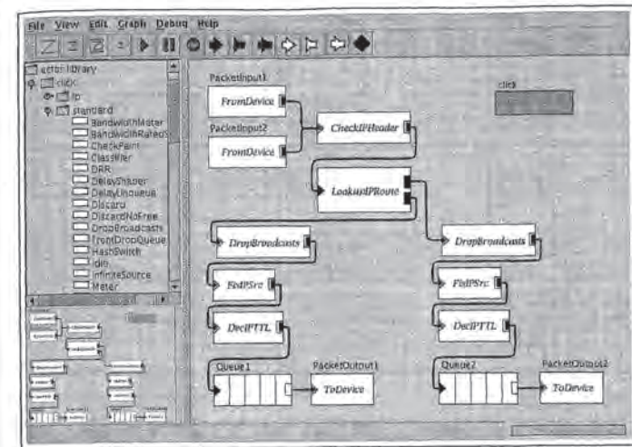
Figure 3.11. Simplified Click Router Application
