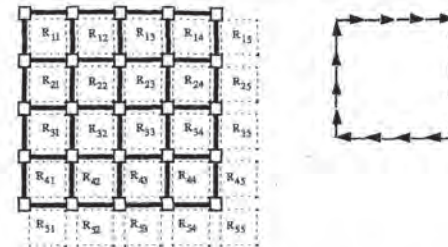
Figure 8.13. Accumulation of clock phase along the NoC. Data is adding a relative phase of +1 T_d travelling down-stream and subtracting -1 T_d travelling up-stream.
