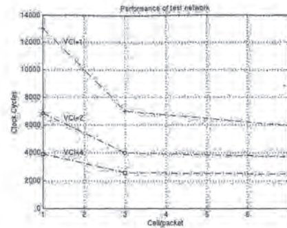
Figure 10.11. Performance of a bidirectional network with different payloads.
