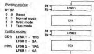
Figure 7. BILBO architecture
