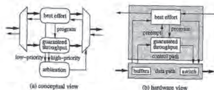
Figure 4.7. Two views of the combined GT-BE router.
