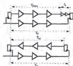
Figure 8.15. Up-stream and down-stream travelling of data.
