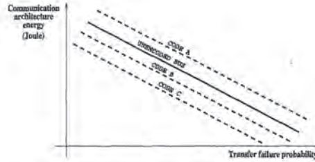
Figure 6.3. Reliability versus energy efficiency for redundant bus encoding schemes making use of low swing signaling.
