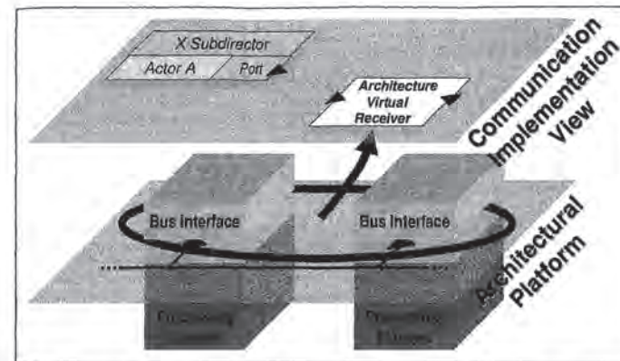
Figure 3.5. Exporting Virtual Receivers
