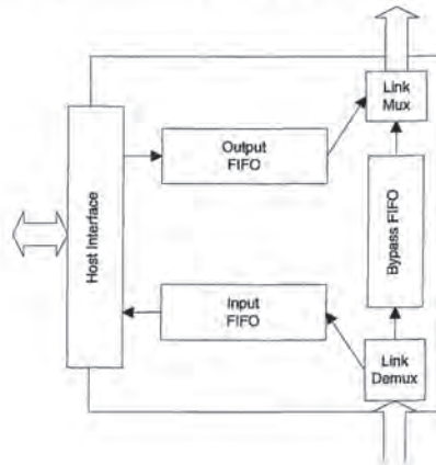
Figure 10.5. Basic Node Architecture.
