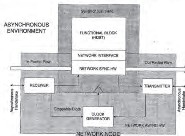
Figure 10.2. Network Node Architecture.
