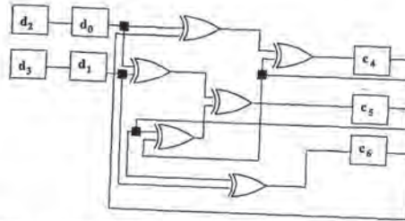
Figure 6.2. Serial-parallel PBCG implementation executing in 2 clock cycles. The transition matrix is raised to the power 2.
