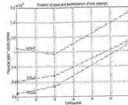
Figure 10.13. Product of area and performance in 2 layered network with different payloads.
