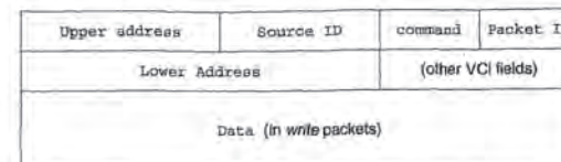
a) Request packet format.
