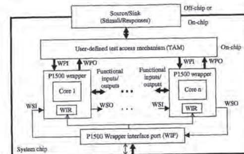
Figure 15. Scalable core test architecture
