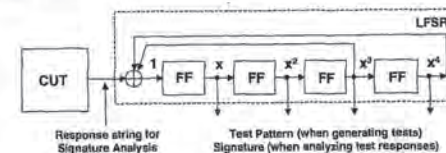
Figure 5. Linear Feedback Shift Register (LFSR)
