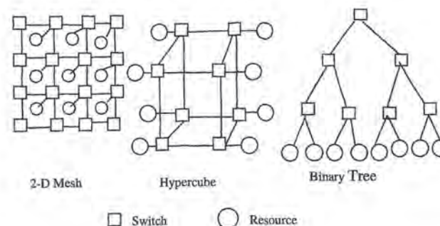
Figure 4: Typical Network Topologies
