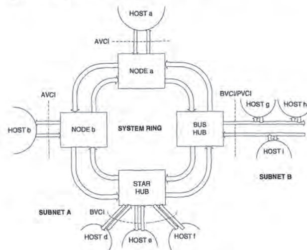
Figure 10.3. Example Proteo network topology.
