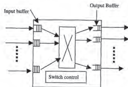
Figure3: A Generic Switch
