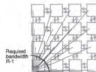
Figure 9-1. Congestion of messages in a machine using simple interleaving occur, if e.g. the size of records equals the number of resources R and the records are accessed in parallel.
