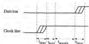
Figure 8.14. Earliest allowed arrival for down-stream travelling data.
