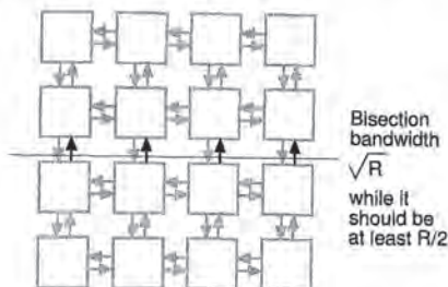
Figure 9-2. The bisection bandwidth of a 2D mesh used in NOC2 is not enough for randomized communication ( R =number of processor resources).
