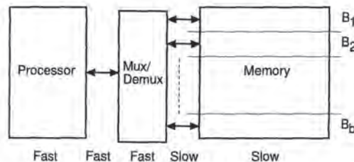
Figure 9-4. A fast stream of references in is divided almost evenly into multiple slow streams that can be handled efficiently by slow memory banks.
