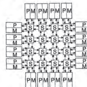
Figure 9-8. A two-dimensional coated mesh (P=processor, M=memory module, S=switch).
