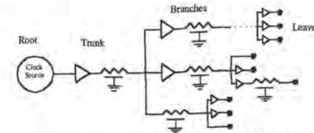
Figure 8.2. Tree structure of a general Clock Distribution Network
