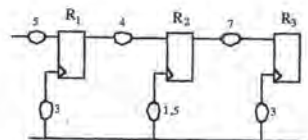
Figure 8.3. Inserting local delay to retime signal-clock skew in data paths.
