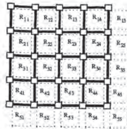
Figure 8.10. An example Network-on-Chip, with 5x5 resources connected together via a 5x5 network of switches.
