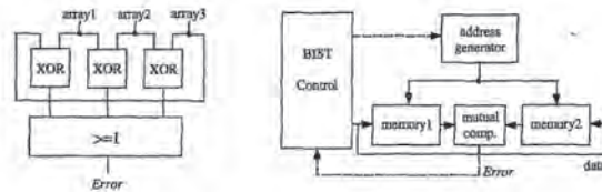
Figure 13. Mutual comparator and its application in MBIST
