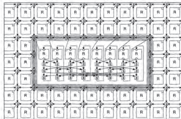
Figure 9-3. A region inside a NOC rounded by the wrapper (S=switch, R=resource).
