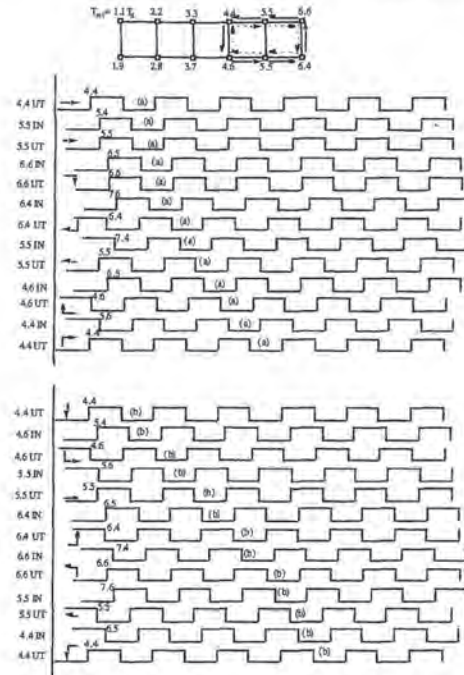
Figure 8.16. Simulation of Time dilation/whirl effects using a Fully Mesochronous clock distribution. a) Clock-wise going message. b) Counterclockwise going message.
