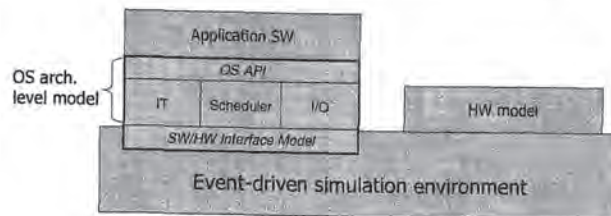
Figure 10 OS architecture level model and simulation environment.
