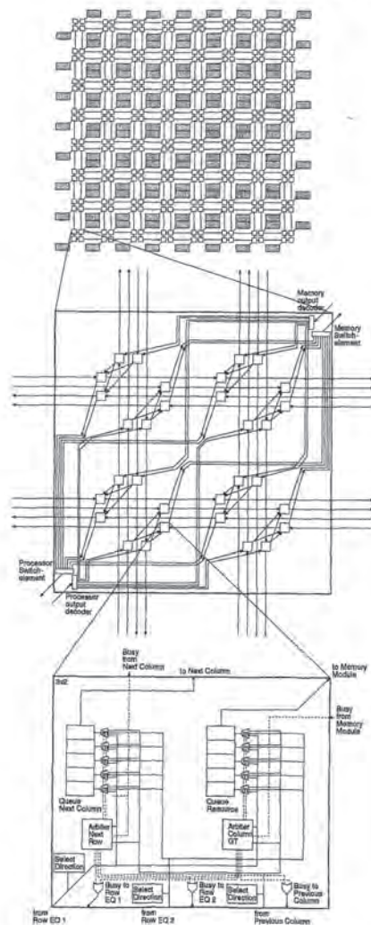
Figure 9-9. A block diagram of an ECLIPSE communication network (top), superswitch (middle), and switch element (bottom).
