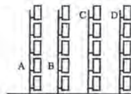
Figure 8.8. Hataminian's and Cash's Clock distribution network of a multiplier array. The difference in skew between A and B and between C and D is almost the same.
