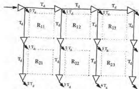
Figure 8.12. The difference in skew between any two neighbouring regions become 1 T_d .
