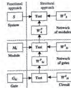
Figure 2. Hierarchical test approach for digital systems
