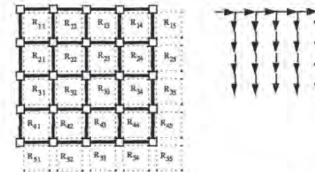
Figure 8.11. The waterfall distribution method with clock entry/source in the upper left corner, with a horizontally distributed waterfall.
