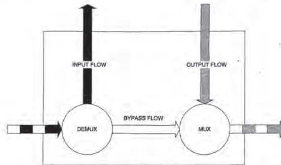
Figure 10.4. Basic node functionality viewed as a mux/demux of packet flows.
