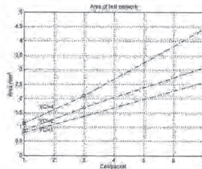
Figure 10.12. Area of 2 layered network with different payloads.
