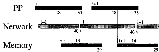
Figure 8: Timeline of optimized transfer of clean lines at the sender.
