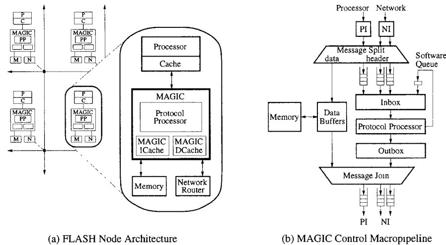
Figure 1: The FLASH architecture.
