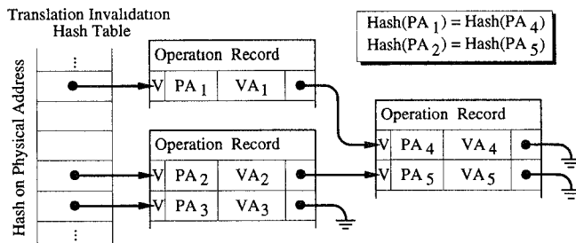
Figure 3: Translation invalidation data structure.
