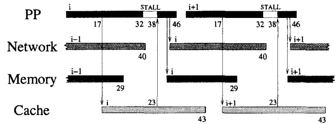
Figure 9: Timeline of optimized transfer of dirty lines at the sender.
