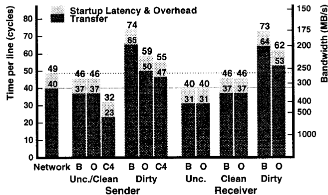
Figure 7: Message transfer performance under various optimizations (32 lines, 10 ns cycles).
