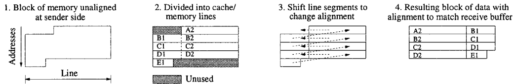
Figure 4: Support for arbitrary user message alignment.
