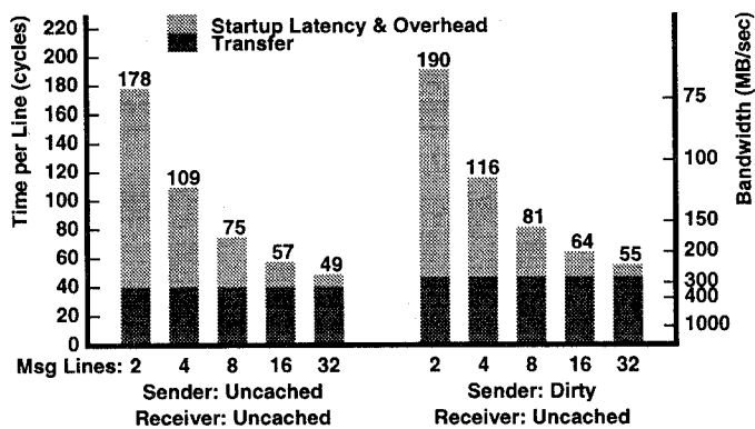
Figure 6: Transfer time per cache line as a function of number of lines (128 byte lines, 10 ns cycles).
