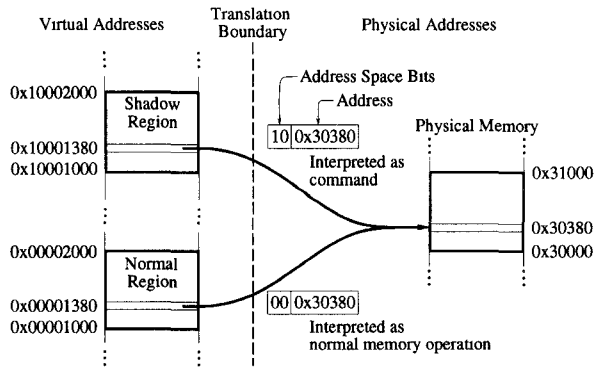
Figure 2: Example of double mapping illustrating the use of alternate physical address spaces.
