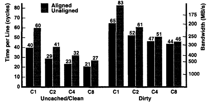
Figure 10: Sender side performance under varying degrees of chunking (32 line transfers).
