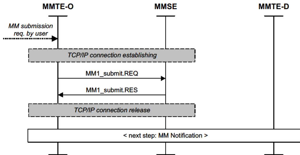
Figure 5: Example abstract message flow for MM Submission
