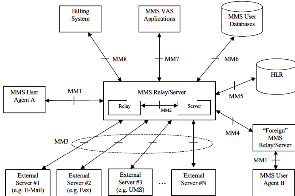
Figure 1: MMS Reference Architecture
