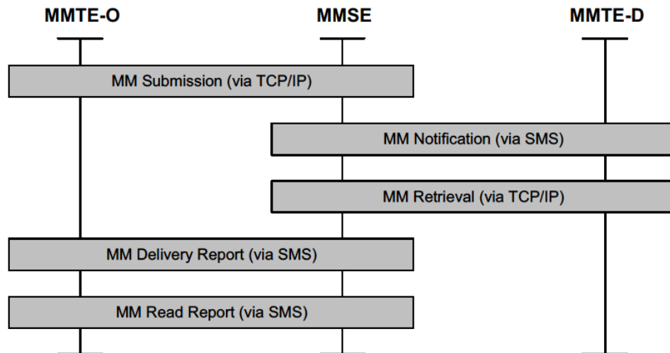
Figure 4: Generalized MMS transaction sequence in fixed networks
