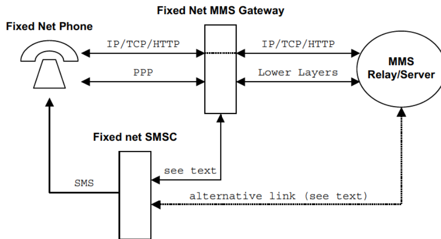
Figure 3: MM1 gateway structure for fixed networks
