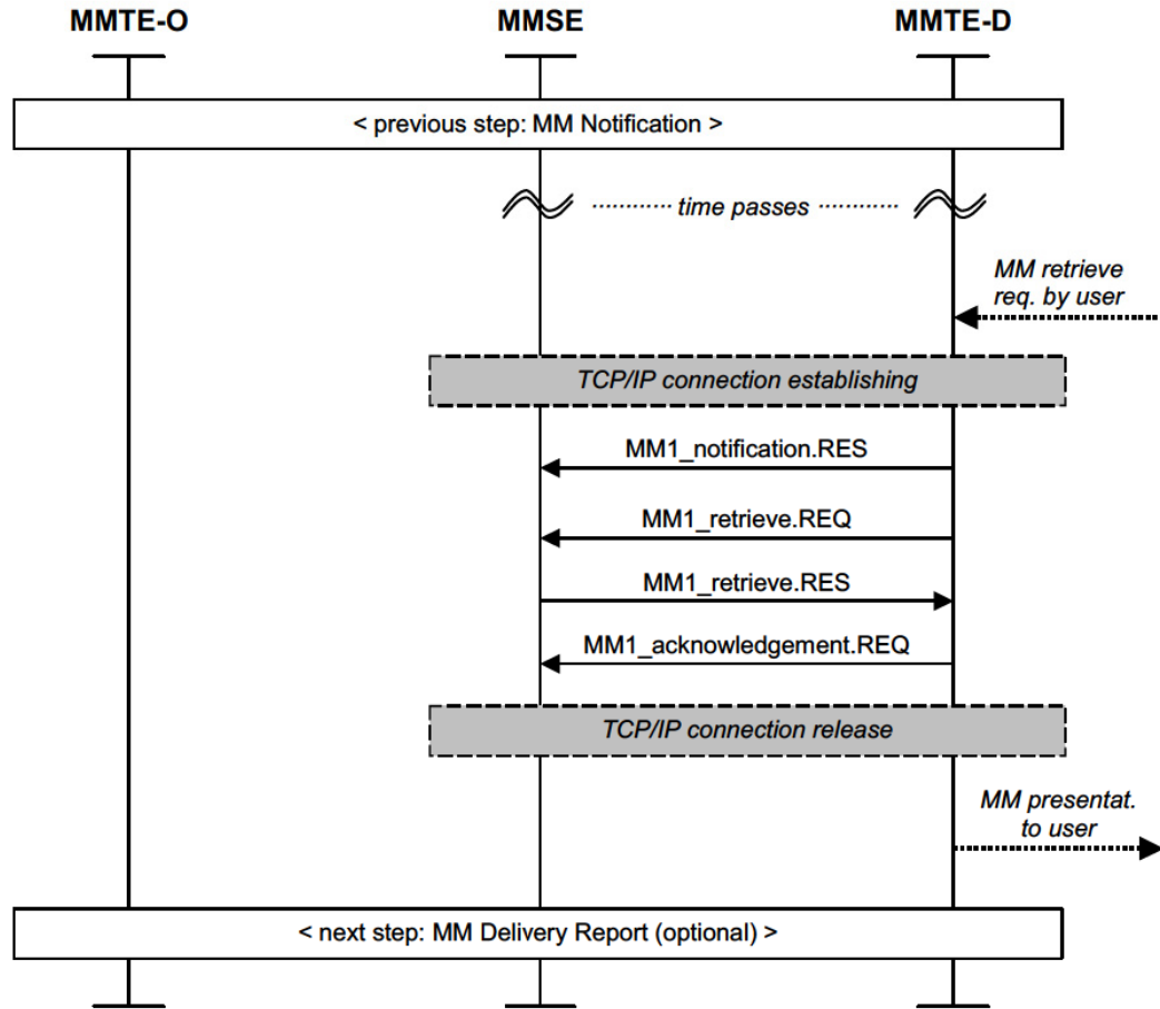
Figure 7: Example abstract message flow for MM Retrieval
