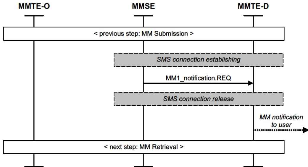
Figure 6: Example abstract message flow for MM Notification
