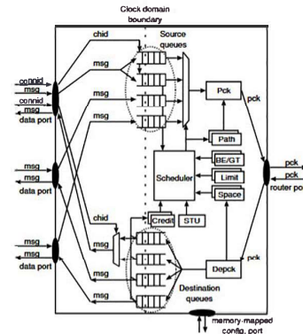
Figure 2. Network interface kernel
