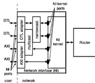
Figure 1. NI kernel and shells
