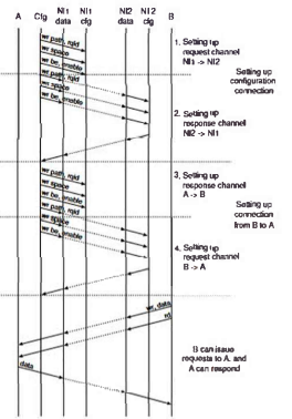
Figure 9. Connection configuration example
