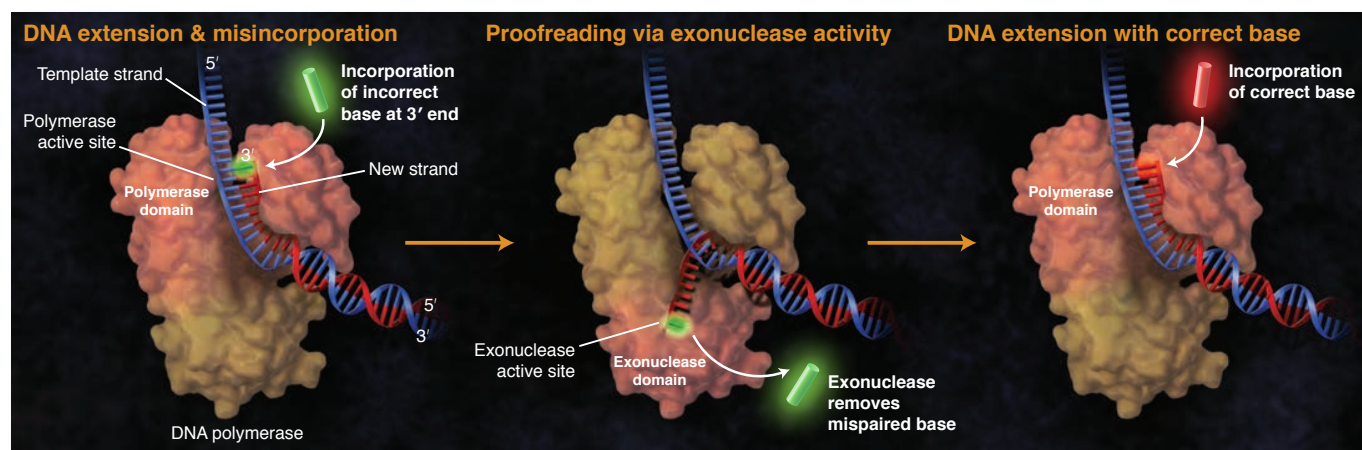
Figure 1. DNA Replication with a Proofreading Polymerase
