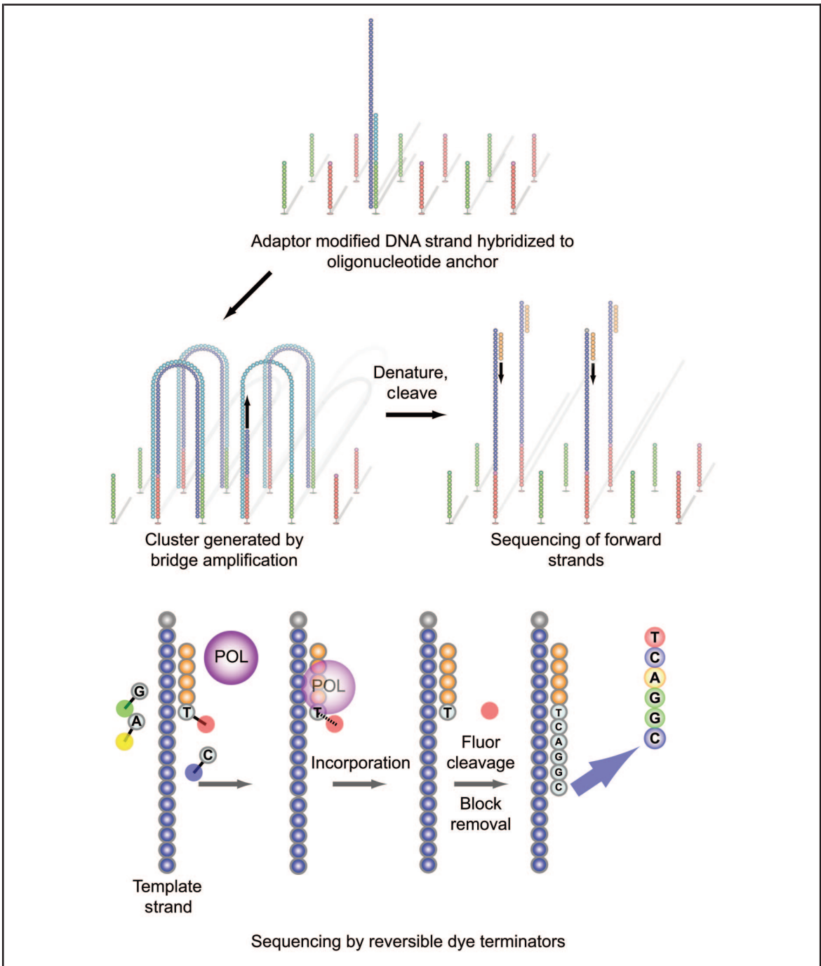
Fig. 2. Illumina Genome Analyzer sequencing. Adapter-modified, single-stranded DNA is added to the flow cell and immobilized by hybridization. Bridge amplification generates clonally amplified clusters. Clusters are denatured and cleaved; sequencing is initiated with addition of primer, polymerase (POL) and 4 reversible dye terminators. Postincorporation fluorescence is recorded. The fluor and block are removed before the next synthesis cycle.
