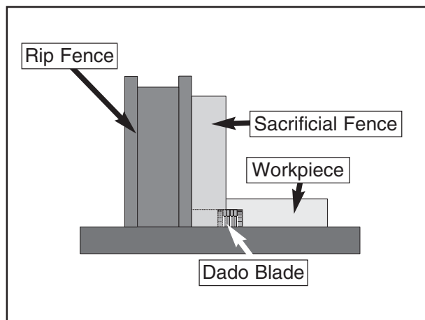
Figure 41. Rabbet cutting.
