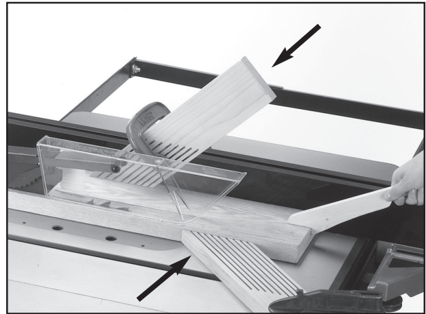
Figure 4. Featherboards in use during a ripping operation.
