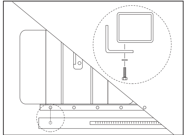
Figure 11. Attaching fence tube to front rail.
