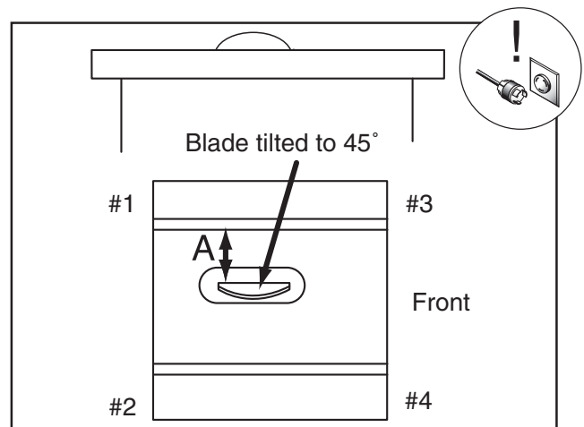
Figure 24. 45° blade parallelism.
