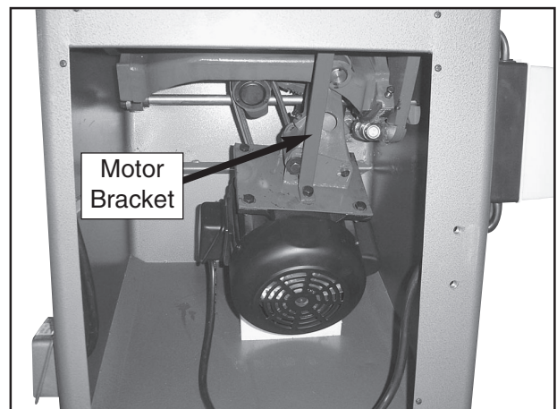
Figure 12. Remove motor bracket.
