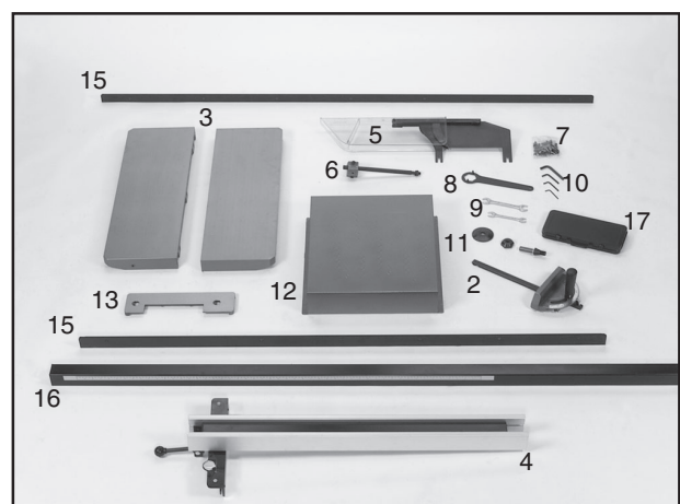
Figure 6. G5959Z component layout.
