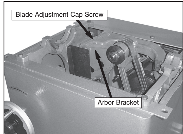
Figure 31. Adjusting arbor bracket.
