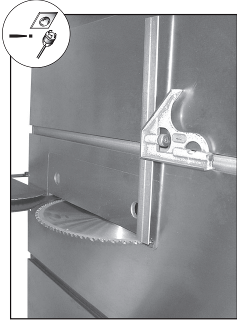
Figure 22. Measuring for parallelism.
