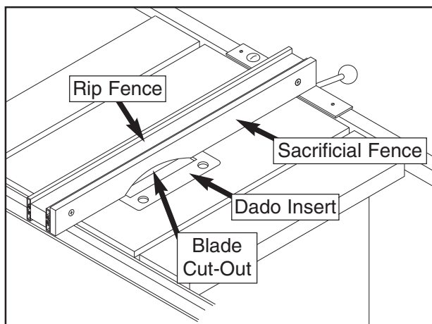
Figure 40. Sacrificial fence.
