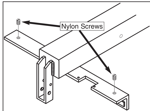
Figure 27. Nylon adjustment screws.
