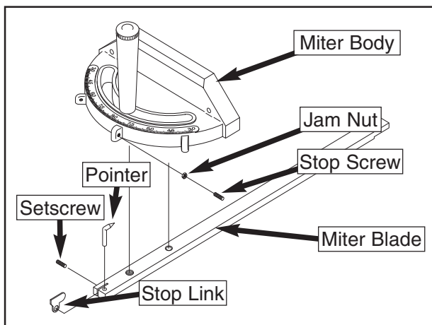
Figure 26. Miter gauge assembly.
