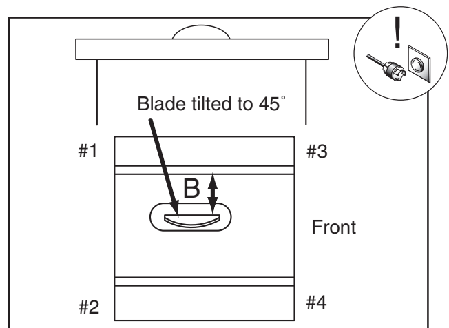
Figure 25. 45° blade parallelism.
