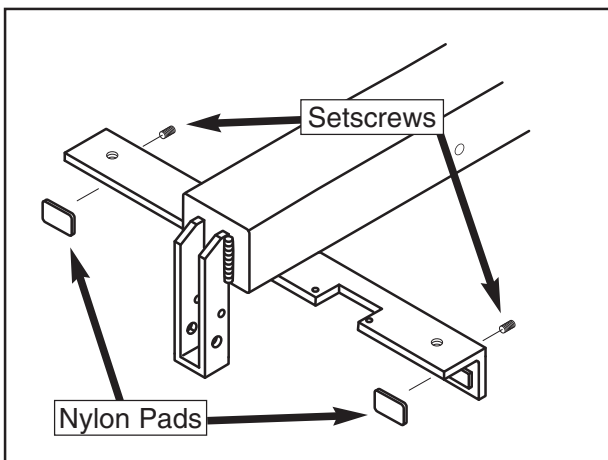
Figure 28. Setscrew adjustments.
