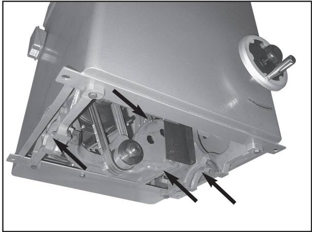
Figure 43. Lubricate these areas.
