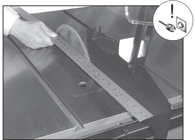
Figure 16. Guard aligned with blade.
