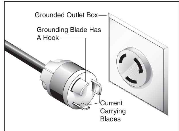
Figure 5. 220V Single-Phase.
