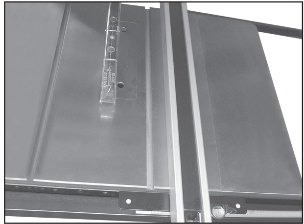
Figure 28. Fence aligned parallel to miter slot.
