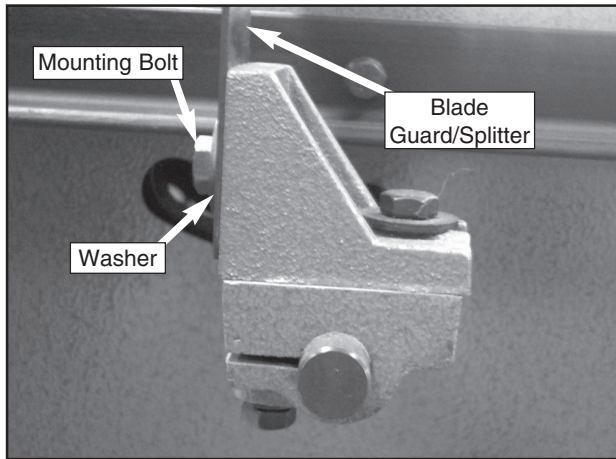
Figure 14. Blade guard and splitter in place.
