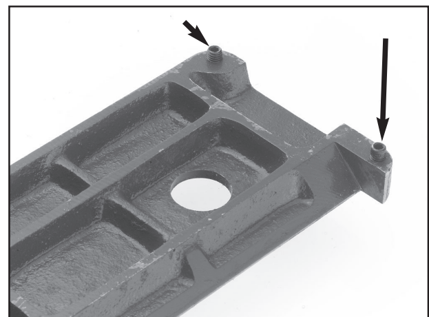
Figure 13. Setscrew on each corner of insert.
