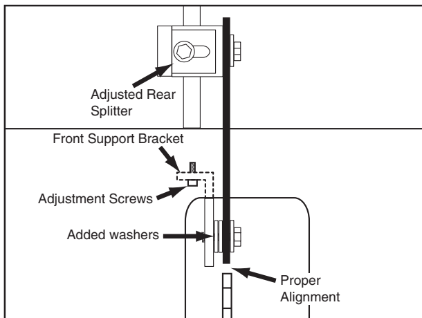
Figure 18. Proper splitter/blade alignment.
