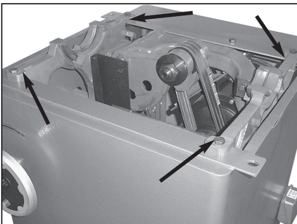
Figure 30. Trunnion mounting bolts.
