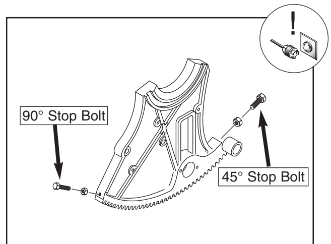
Figure 20. 90° and 45° stop bolts.
