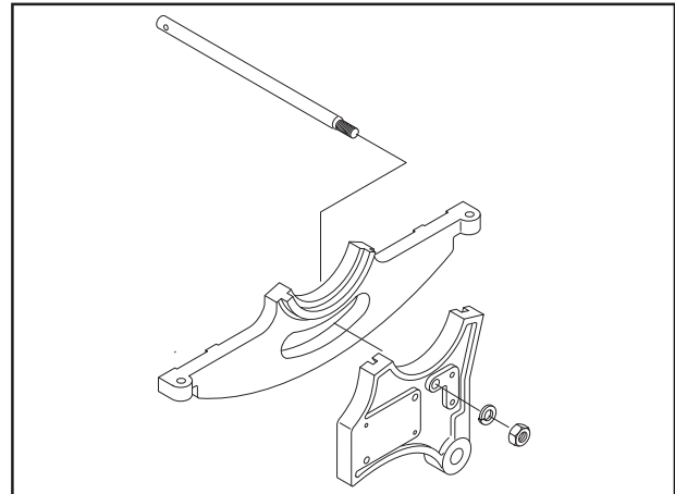
FIGURE 8. Attaching guard support shaft.
