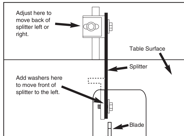
Figure 17. Improper splitter/blade alignment.
