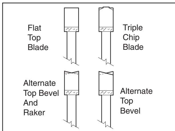
Figure 36. Various saw tooth cutting profiles.
