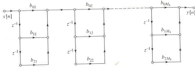
Figure 6.33 Cascade-form realization of an FIR system.
