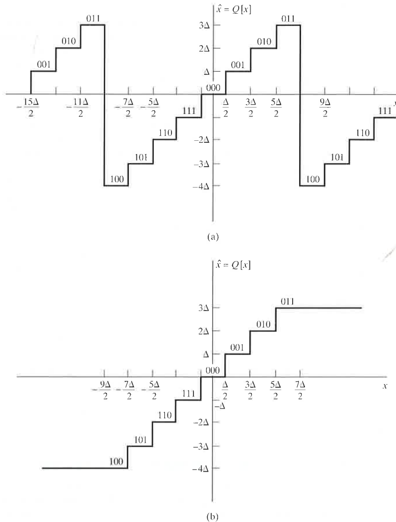
Figure 6.38 Two's-complement rounding. (a) Natural overflow. (b) Saturation.
