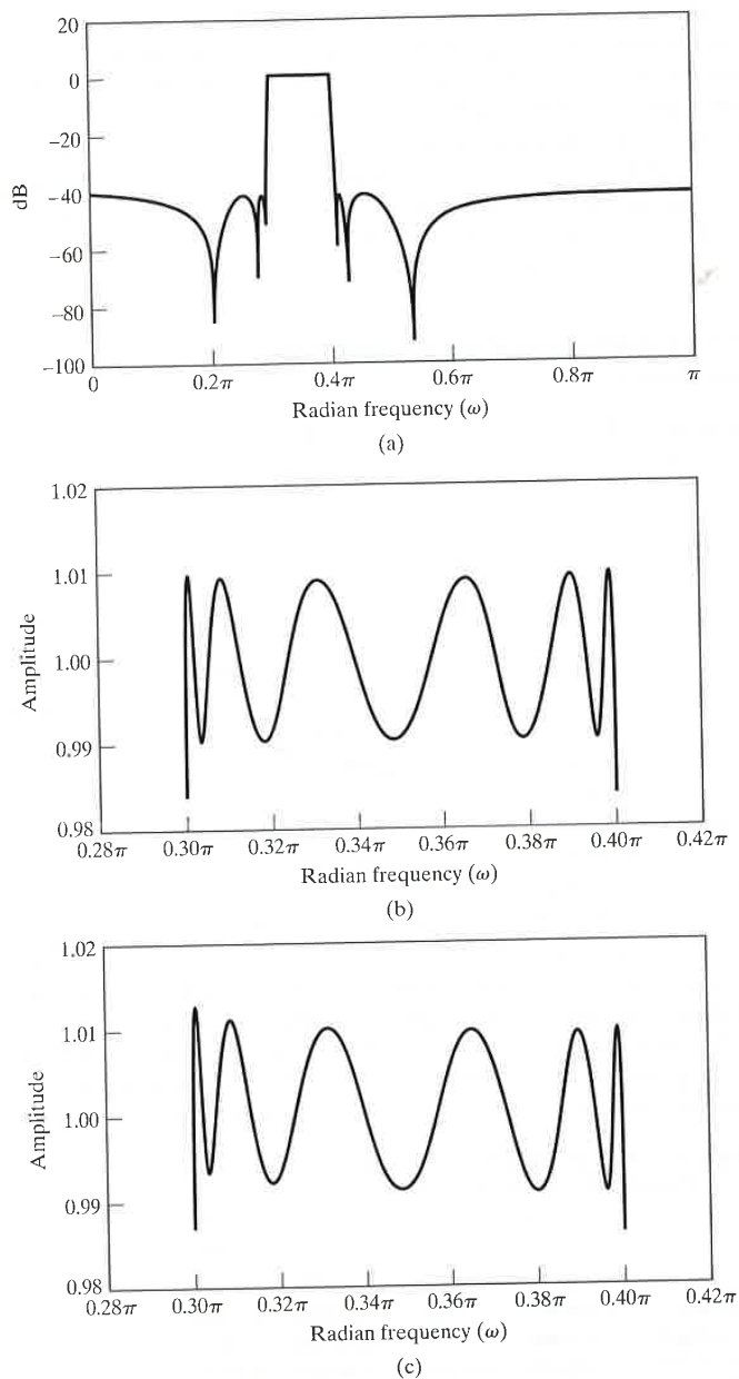
Figure 6.40 IIR coefficient quantization example. (a) Log magnitude for unquantized elliptic bandpass filter. (b) Passband for unquantized cascade case. (c) Passband for cascade structure with 16-bit coefficients.
