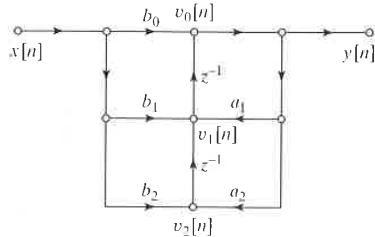
Figure 6.28 Transposed direct form II structure for Example 6.8.
