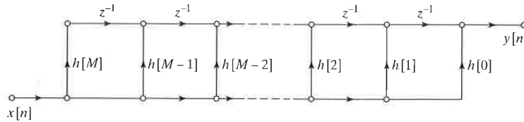
Figure 6.32 Transposition of the network of Figure 6.31.
