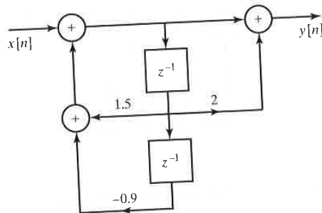
Figure 6.7 Direct form II implementation of Eq. (6.16).
