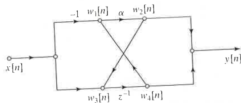
Figure 6.12 Flow graph not in standard direct form.
