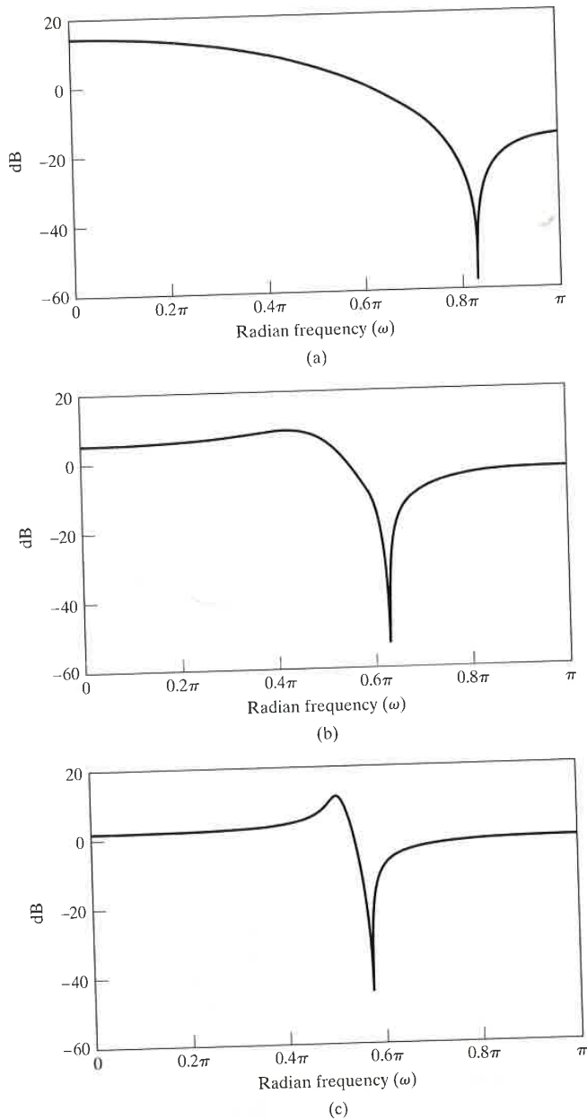
Figure 6.58 Frequency-response functions for example system. (a) 20 \log_{10} |H_1(e^{j\omega})| . (b) 20 \log_{10} |H_2(e^{j\omega})| . (c) 20 \log_{10} |H_3(e^{j\omega})| .
