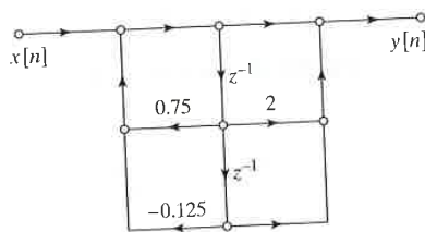
Figure 6.17 Direct form II structure for Example 6.4.
