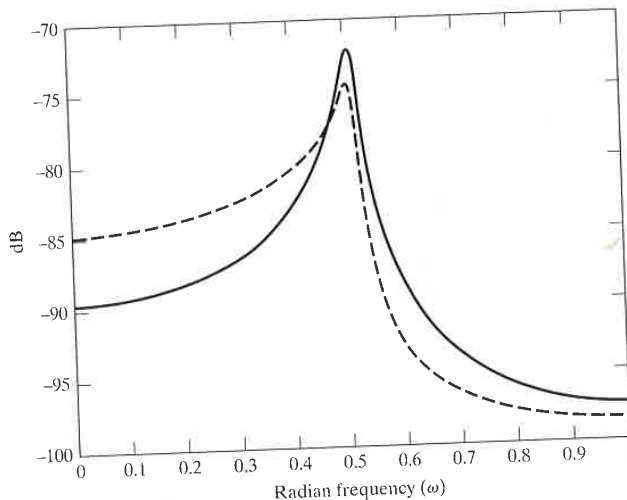
Figure 6.59 Output noise power spectrum for 123 ordering (solid line) and 321 ordering of second-order sections.
