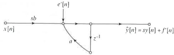
Figure 6.55 Scaled first-order system.
