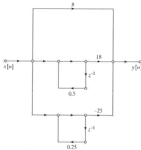
Figure 6.22 Parallel-form structure for Example 6.6 using first-order systems.
