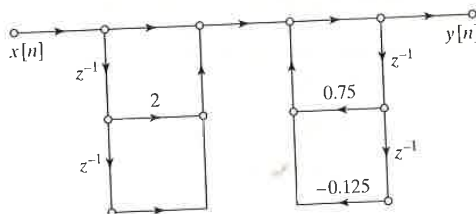
Figure 6.16 Direct form I structure for Example 6.4.
