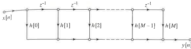
Figure 6.31 Direct-form realization of an FIR system.
