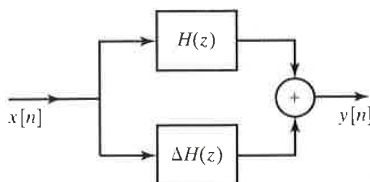
Figure 6.45 Representation of coefficient quantization in FIR systems.
