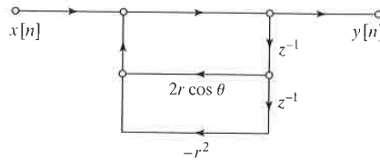
Figure 6.41 Direct-form implementation of a complex-conjugate pole pair.
