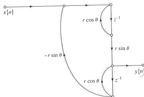
Figure 6.43 Coupled-form implementation of a complex-conjugate pole pair.
