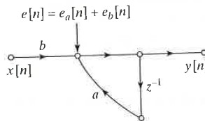
Figure 6.52 First-order linear noise model.
