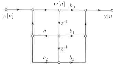
Figure 6.27 Direct form II structure for Example 6.8.
