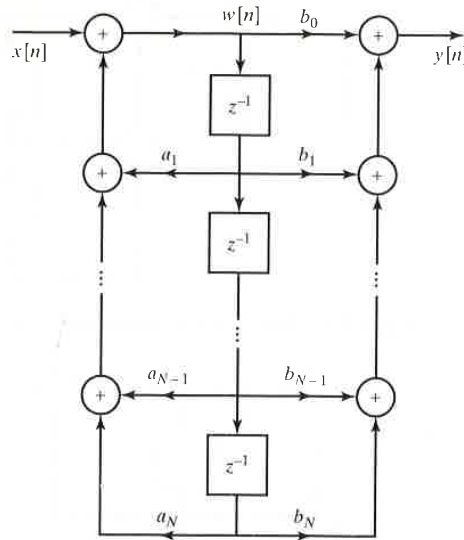
Figure 6.5 Combination of delays in Figure 6.4.
