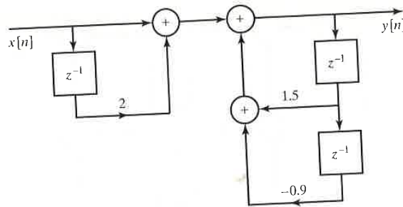
Figure 6.6 Direct form I implementation of Eq. (6.16).
