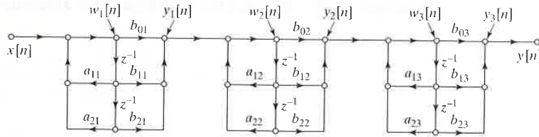
Figure 6.18 Cascade structure for a sixth-order system with a direct form II realization of each second-order subsystem.
