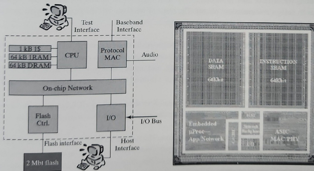
Figure 8-15 Wireless communications processor—an example of a hybrid ASIC design methodology. The processor combines an embedded microprocessor and its memory system with dedicated hardware accelerators and I/O modules. Observe also the on-chip network module [Silva01].
