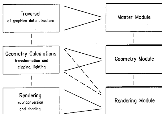
FIGURE 4.1. Mapping functional sections to hardware
