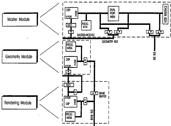
FIGURE 4.2. Basic module structure
