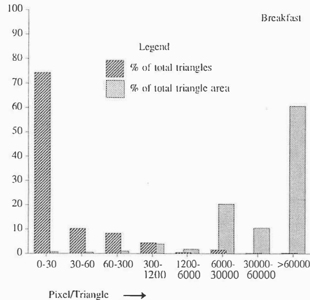
FIGURE 4.6. Image statistics for "breakfast"
