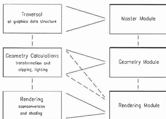
FIGURE 4.1. Mapping functional sections to hardware
