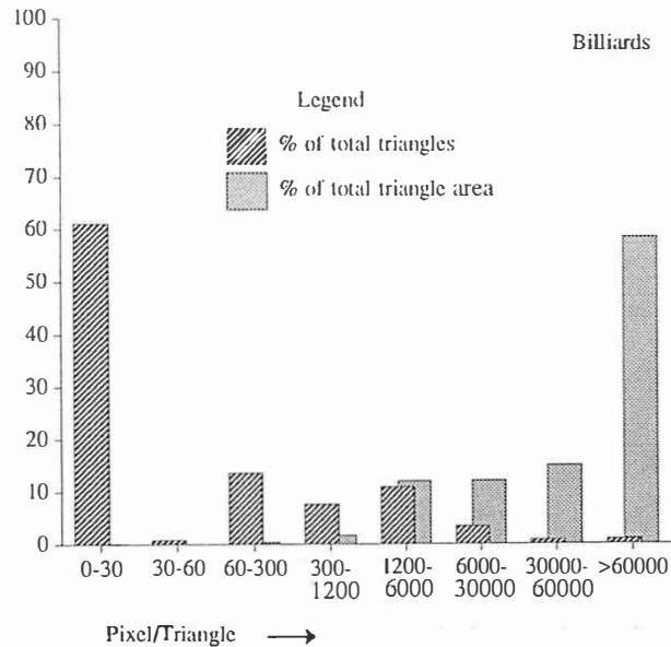
FIGURE 4.7. Image statistics for "billiards"
