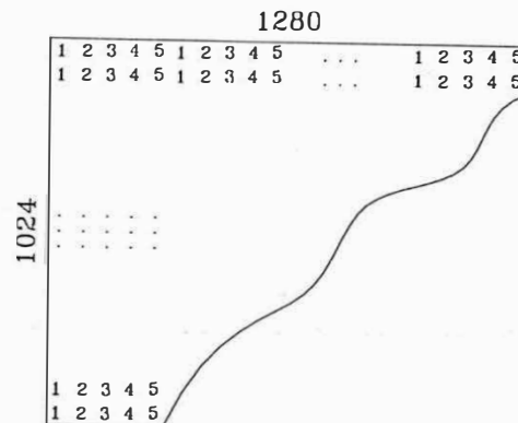
FIGURE 4.3. Frame buffer interleaving
