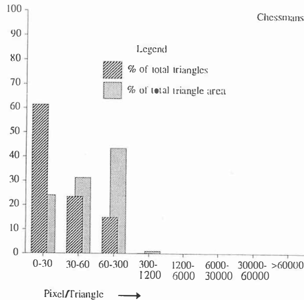
FIGURE 4.8. Image statistics for "chessmen"
