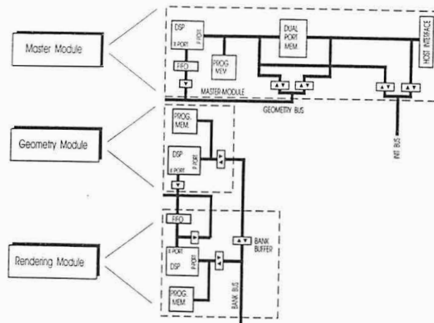
FIGURE 4.2. Basic module structure
