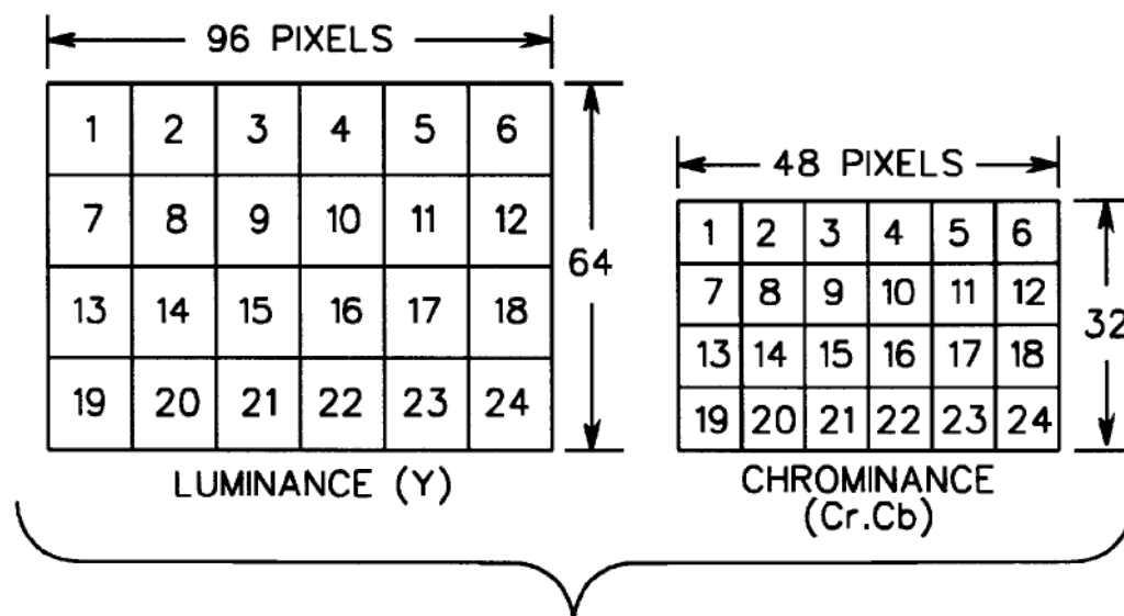
fig. 2 (PRIOR ART)
