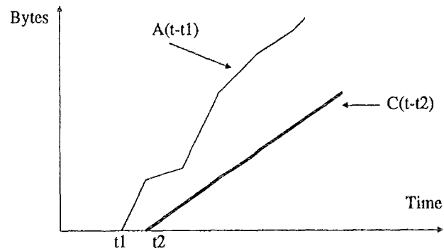
Fig.4 Average arriving rate is larger than the output rate, buffer requirement becomes larger and larger with time
