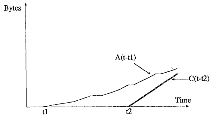
Fig.5 Average arriving rate is smaller than the output rate, there is a long initial delay and large buffer requirement
