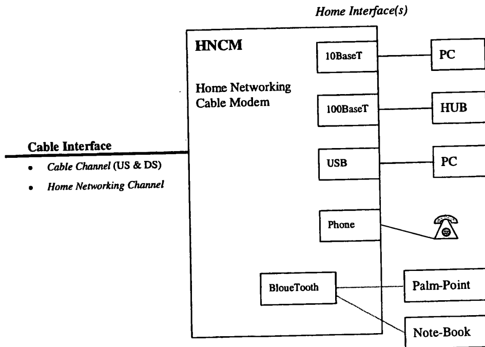
Figure 8: HCNM Data Channels
