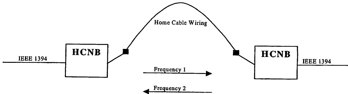
Figure 12: Layer Two Transporting over Home Networking
