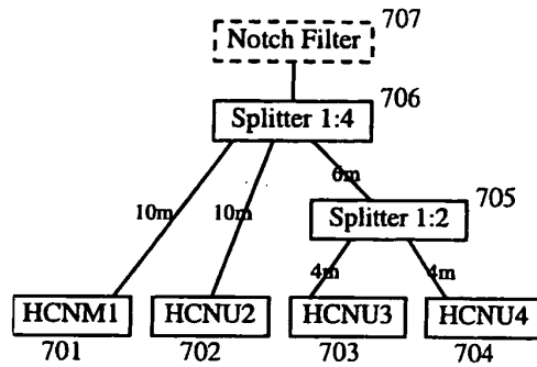
Figure 7: Example of home wiring that contain notch filter
