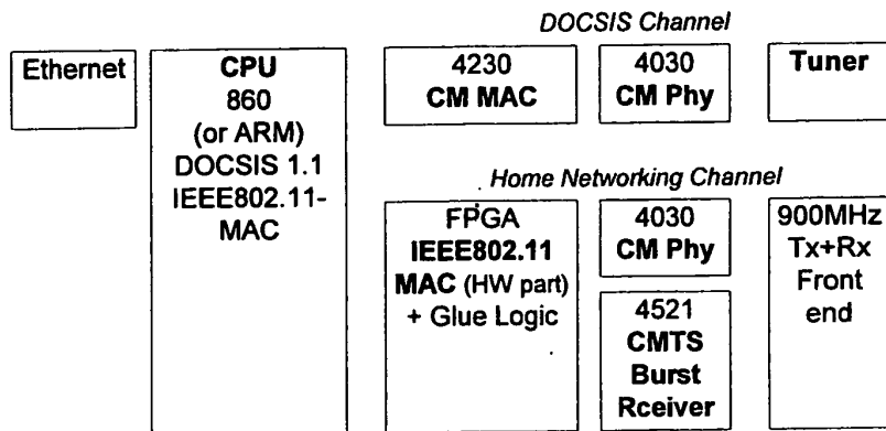
Figure 19: HCNM Proof Of Concept – Card
