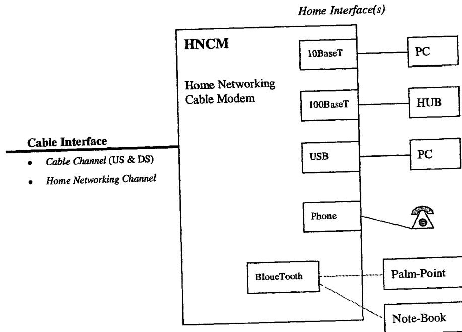
Figure 8: HCNM Data Channels
