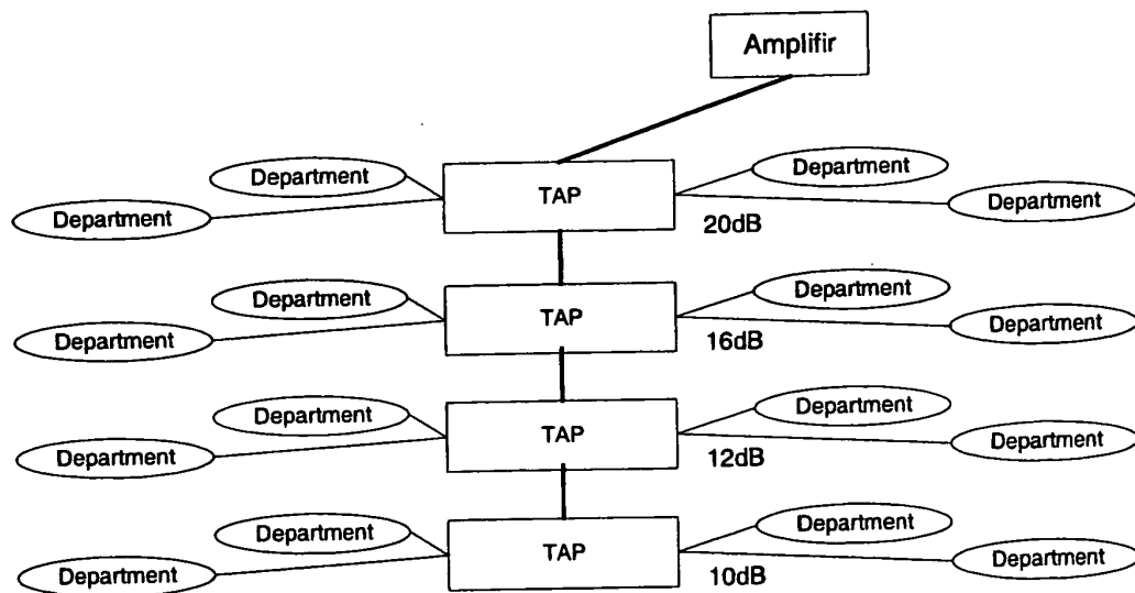
Figure 15: Wiring in big department building
