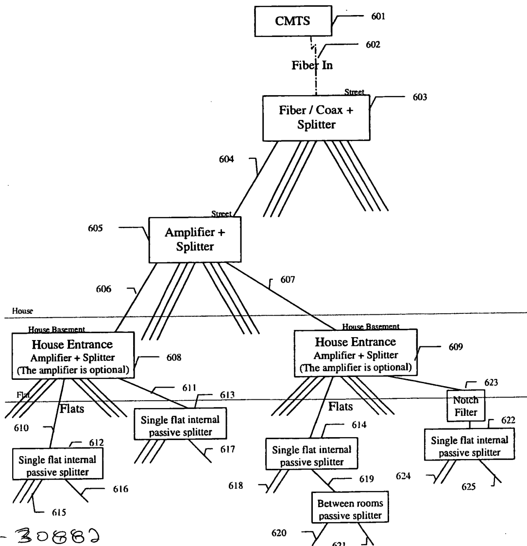
Figure 6: HFC infrastructure
