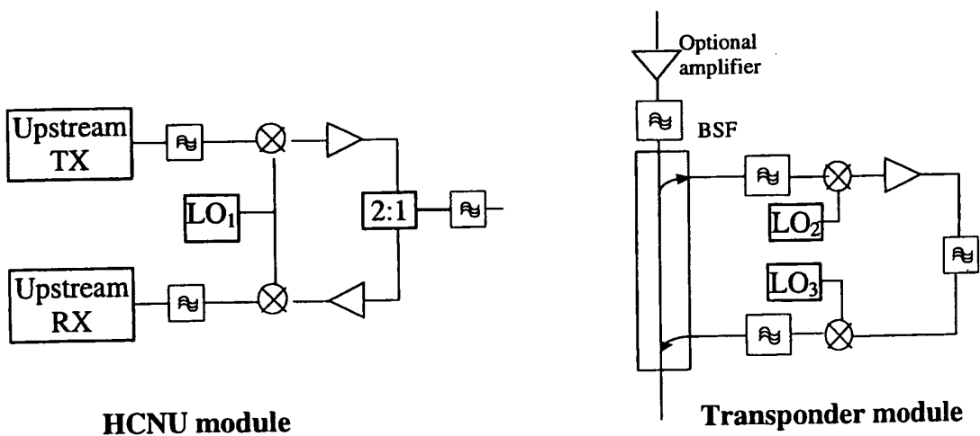
Figure 11: Dual Frequencies Mode components
