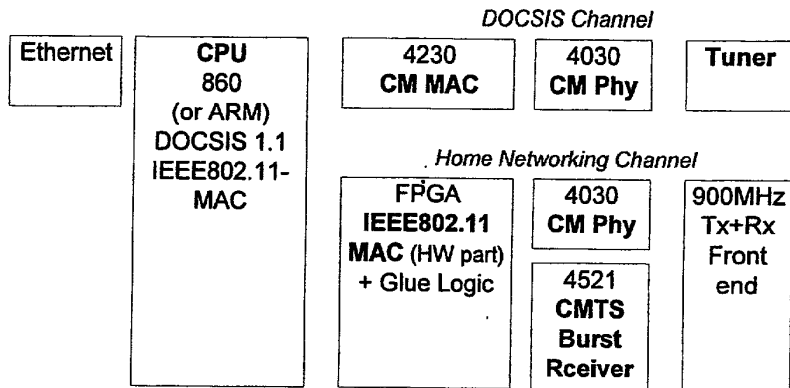
Figure 19: HCNU Proof Of Concept – Card
