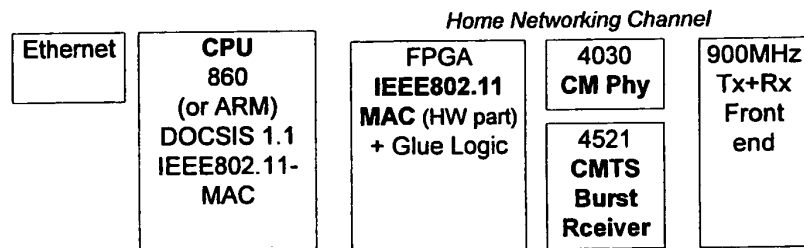
Figure 19: HCNM Proof Of Concept – Card
