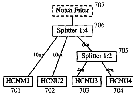
Figure 7: Example of home wiring that contain notch filter
