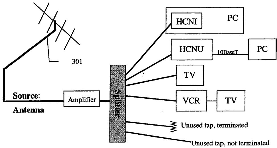
Figure 3 – HomeCN connected to a TV antenna
