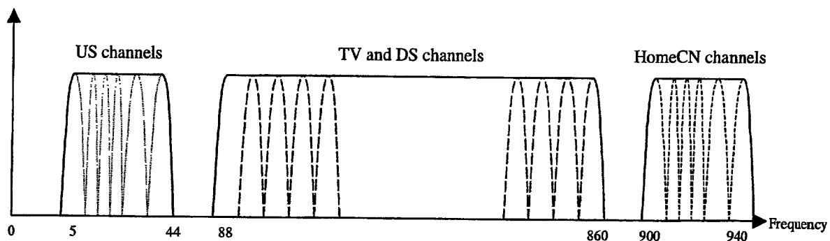
Figure 5 – Frequency Allocation
