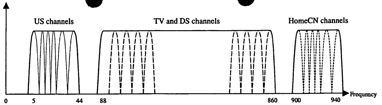
Figure 5 – Frequency Allocation
