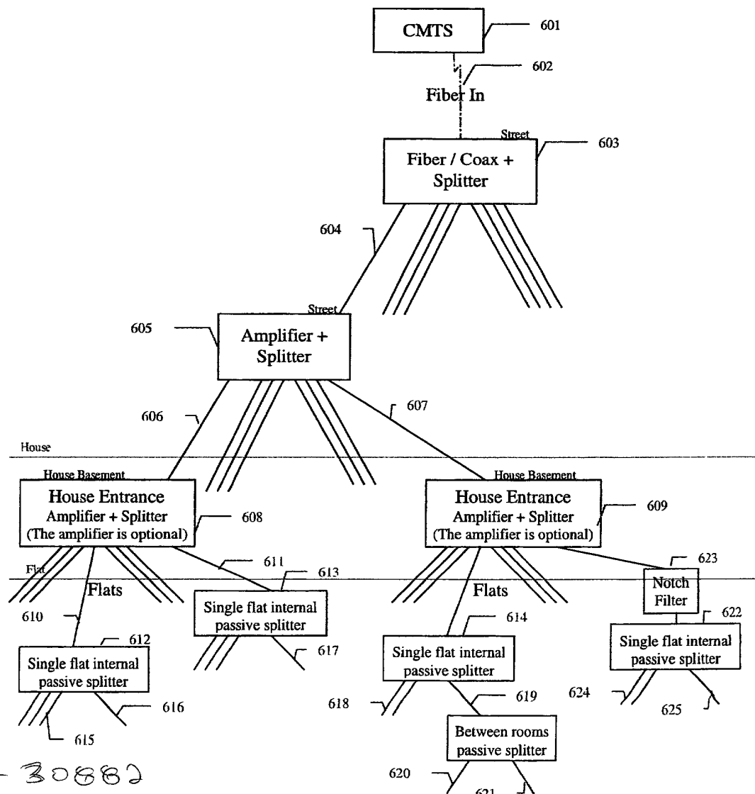
Figure 6: HFC infrastructure
