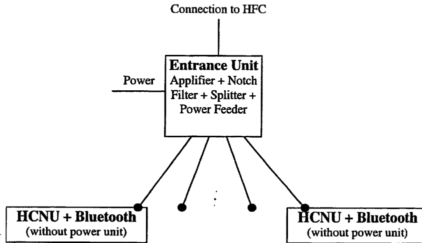
Figure 10: Central Power Supply
