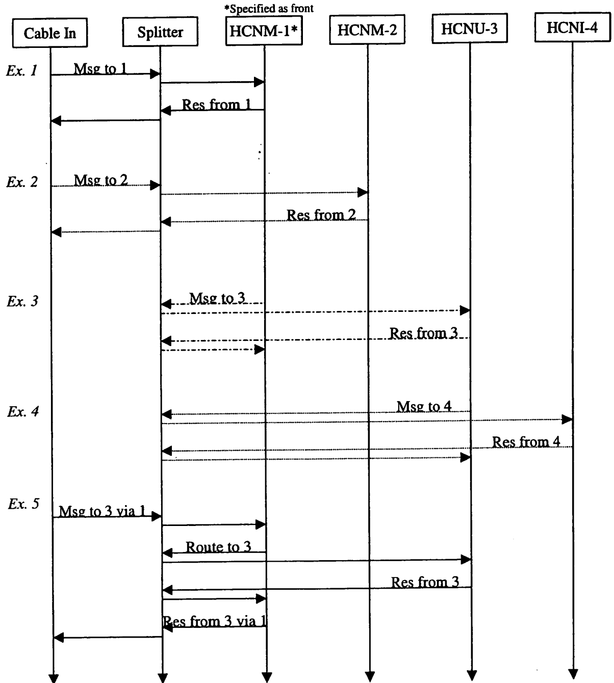
Figure 9 – HomeCN data flow examples
