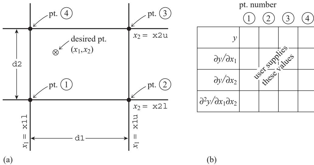
Figure 3.6.1. (a) Labeling of points used in the two-dimensional interpolation routines bcuint and bcucf . (b) For each of the four points in (a), the user supplies one function value, two first derivatives, and one cross-derivative, a total of 16 numbers.
