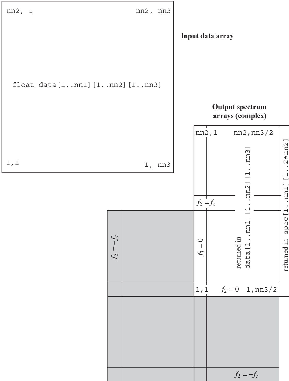
Figure 12.5.1. Input and output data arrangement for rlft3 . All arrays shown are presumed to have a first (leftmost) dimension of range [1..nn1] , coming out of the page. The input data array is a real, three-dimensional array data[1..nn1][1..nn2][1..nn3] . (For two-dimensional data, one sets nn1 = 1 .) The output data can be viewed as a single complex array with dimensions [1..nn1][1..nn2][1..nn3/2+1] (cf. equation 12.5.3), corresponding to the frequency components f_1 and f_2 being stored in wrap-around order, but only positive f_3 values being stored (others being obtainable by symmetry). The output data is actually returned mostly in the input array data , but partly stored in the real array speq[1..nn1][1..2*nn2] . See text for details.
