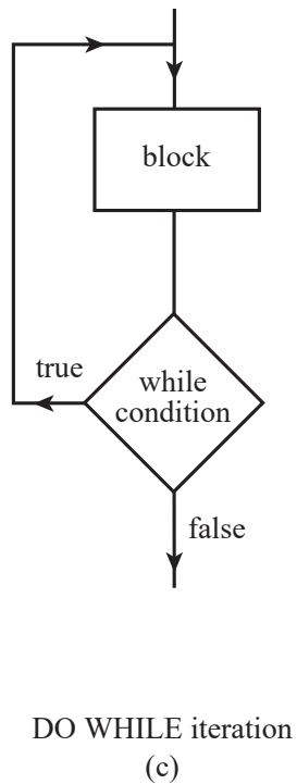
Figure 1.1.1. Standard control structures used in structured programming: (a) for iteration; (b) while iteration; (c) do while iteration; (d) break iteration; (e) if structure; (f) switch structure
