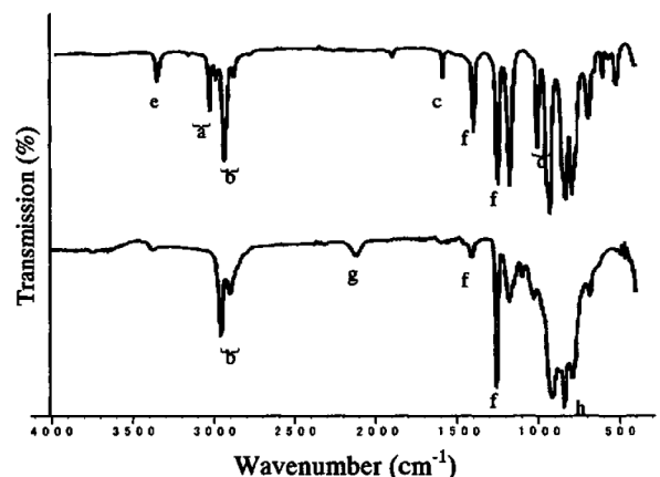
Figure 5. FT-IR transmission spectrum of 1,1,3,3-tetramethyl-1,3-divinyldisilazane monomer (top) and its pp-film (bottom). Assignment of the IR absorption band are as follows: a; =C-H stretch, b; C-H stretch, c; C=C stretch, d; C-H out of plane bend, e; N-H stretch, f; Si-CH 3 vibration, g; Si-H stretching and h; Si-H bend.
