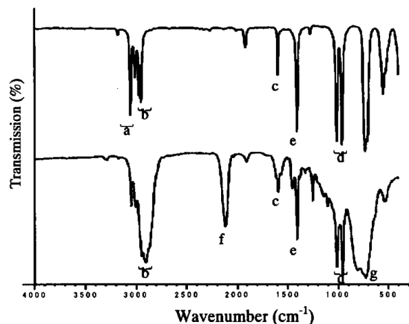
Figure 9. FT-IR transmission spectra of tetravinylsilane monomer (top) and its pp-film (bottom). Assignment of the IR absorption bands are as follows: a; =C-H stretch, b; C-H stretch, c; C=C stretch, d; C-H out of plane bend, e; Si-CH 3 vibration, f; Si-H stretching and g; Si-H bend.
