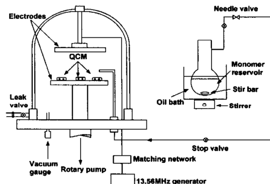
Fig. 1a. Schematic of the plasma polymerization equipment.
