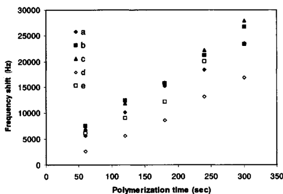
Figure 2. Frequency shift of QCMs in relationship to the polymerization time for the various positions on the lower electrode for 1,3-divinyldimethyltetramethyldisiloxane.
