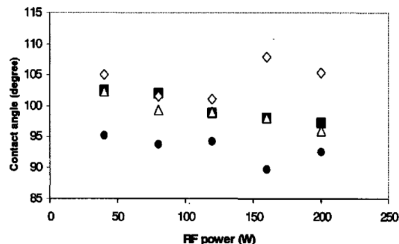
Figure 13. Contact angles of water for pp-films of 1,3-divinyldimethylsiloxane (■), 1,1,3,3-tetramethyl-1,3-divinyldisilazane (●), tetravinylsilane (◇) and diallyldimethylsilane, (△) as a function of RF power.
