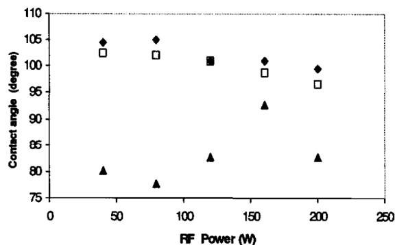
Figure 12. Contact angles of water for pp-films of allyltrimethylsilane (◆), vinyltrimethylsilane (□) and vinyltriethoxysilane (▲) as a function of RF power.
