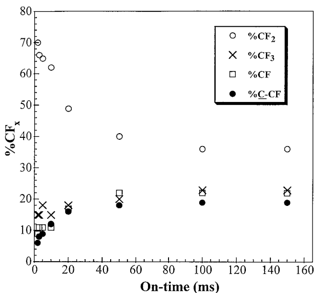
Figure 7 The composition of pulsed PECVD films as a function of on-time holding the off-time fixed at 400 ms. The flow rate was fixed at 12.5 sccm and default values (Table I) were used for the other process conditions. The %CF 2 decreases with on-time until a constant value of 36% is reached.
