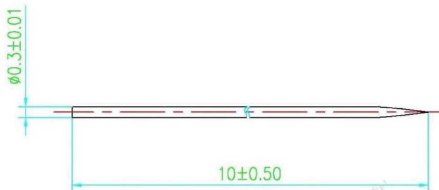
2. Needle (unit: mm)
