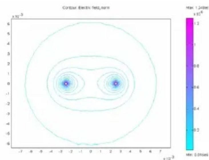
Fig. 5: Electric Field Distribution due to Needle Electrode Configuration
