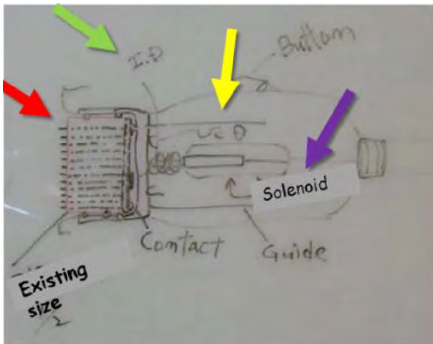
Figure 2: Hand Drawing of Proposed Fully Automatic RF MTS with Annotations by Mr. Kim
