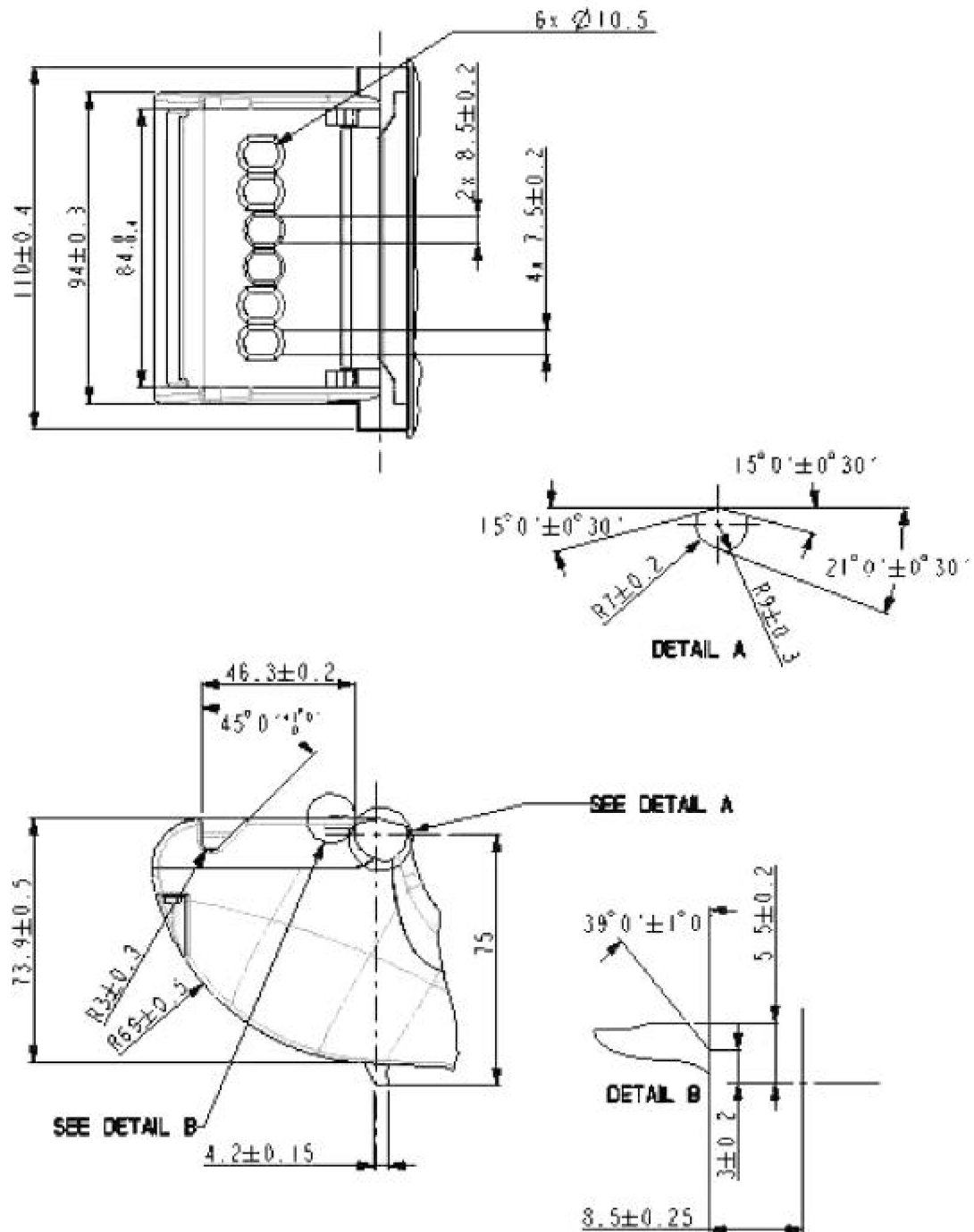
FIGURE 10—CONNECTOR PHYSICAL CONTROL DIMENSIONS
