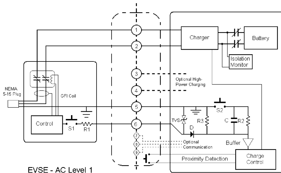
FIGURE 4—AC LEVEL 1 SYSTEM CONFIGURATION
