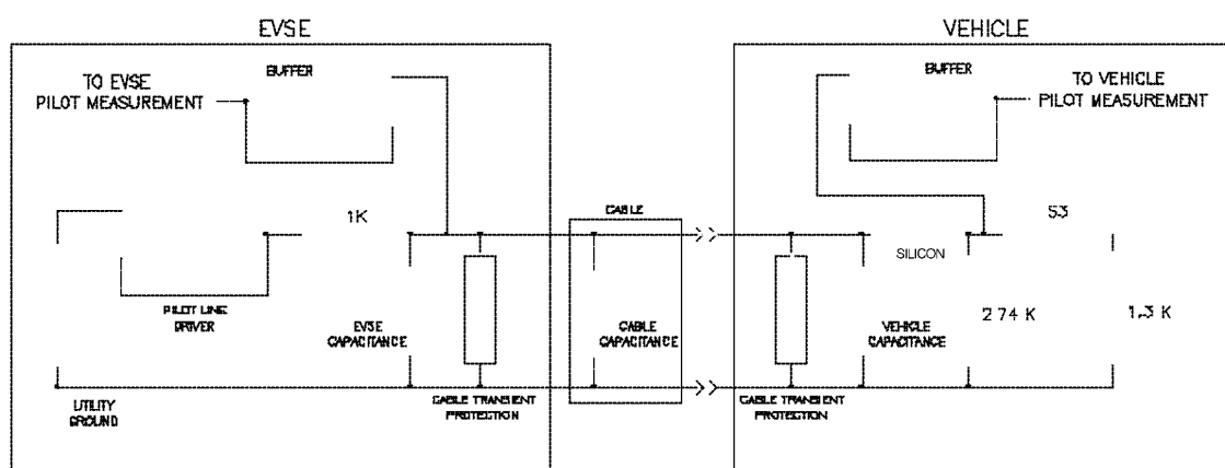
FIGURE A1—TYPICAL PILOT LINE CIRCUITRY
