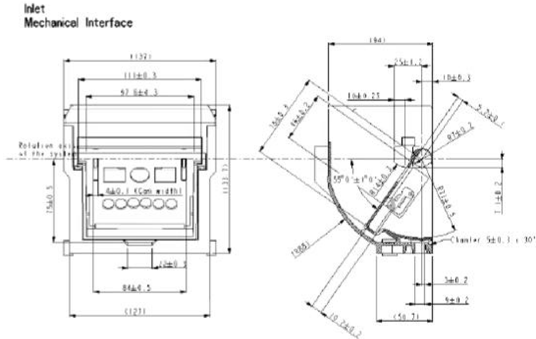
FIGURE 11—VEHICLE INLET PHYSICAL CONTROL DIMENSIONS
