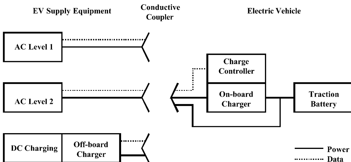
FIGURE 1—CONDUCTIVE EV CHARGING SYSTEM ARCHITECTURE
