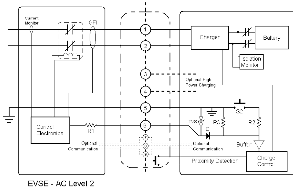
FIGURE 3—AC LEVEL 2 SYSTEM CONFIGURATION
