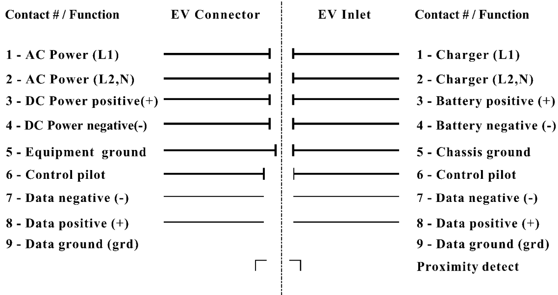
FIGURE 2—CONDUCTIVE COUPLER CONTACT INTERFACE FUNCTIONS
