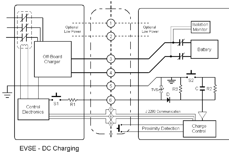
FIGURE 5—DC CHARGING SYSTEM CONFIGURATION
