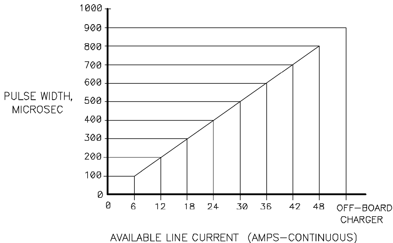
FIGURE 8—EVSE CURRENT CAPACITY VERSUS CONTROL PILOT PULSE WIDTH
