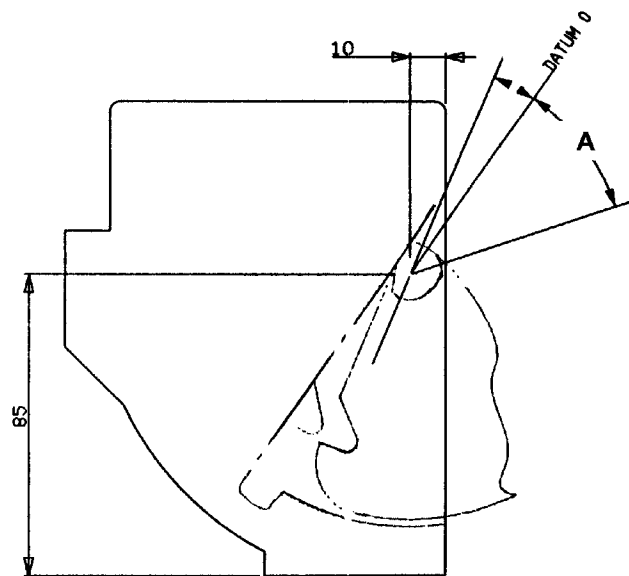
FIGURE 13—COUPLER INTERFACE CONTACT SEQUENCING
