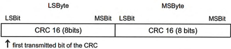
Figure 3 — CRC bits and bytes transmission rules
