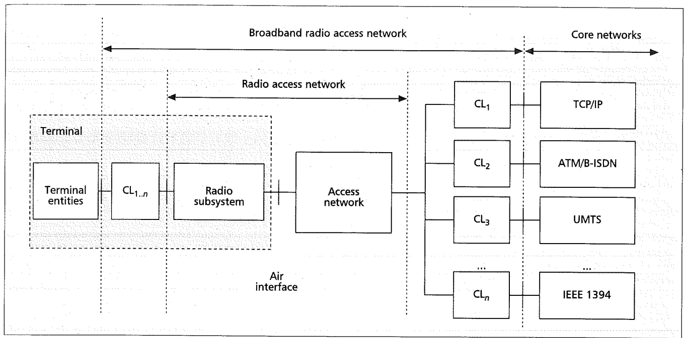
■ Figure 1. The HIPERLAN/2 reference model [2].
