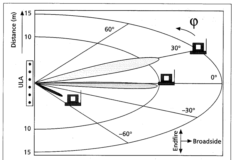
■ Figure 2. Simultaneous transmission using directive beams.
