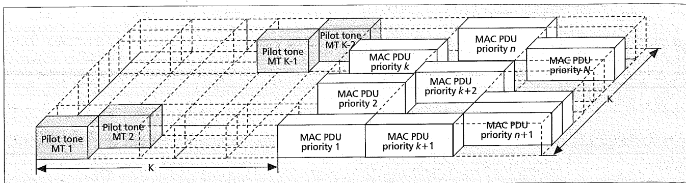
■ Figure 5. Uplink space time schedule for K associated MTs.
