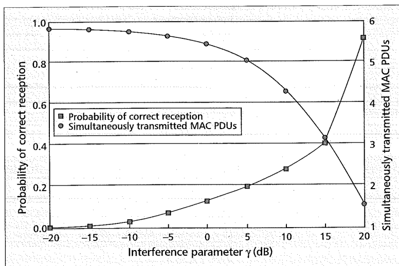
■ Figure 6. Successful reception and spatial exploitation.
