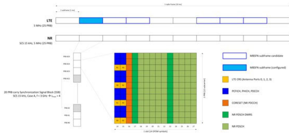
Figure 1 NR signal configuration within the MBSFN subframe.
