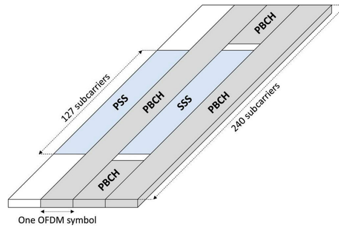
Figure 16.1 Time/frequency structure of a single SS block consisting of PSS, SSS, and PBCH.
