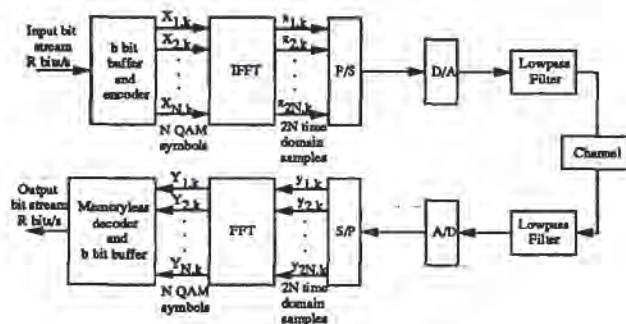
Figure 1: DMT block diagram
