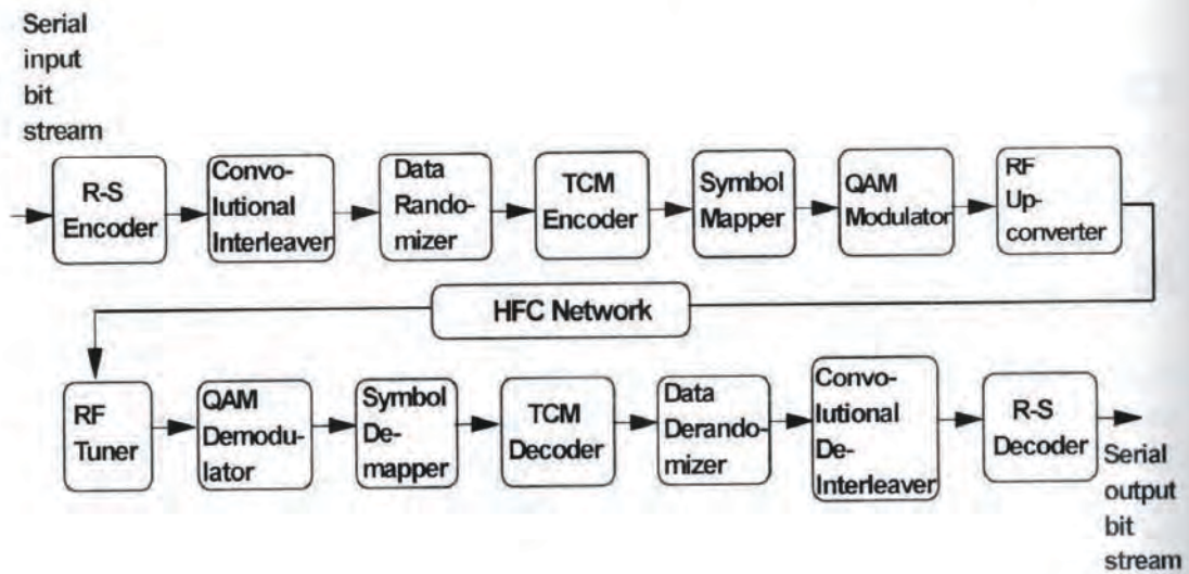
Figure 7.1 A simplified block diagram of RF QAM modem operating over HFC network.
