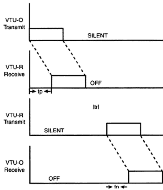
Figure 9.11 An example of TDD.
