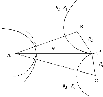
Fig. 2. Positioning based on TDOA measurements.
