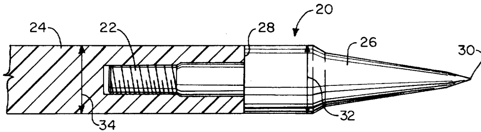
FIG. 1 KNOWN ART
