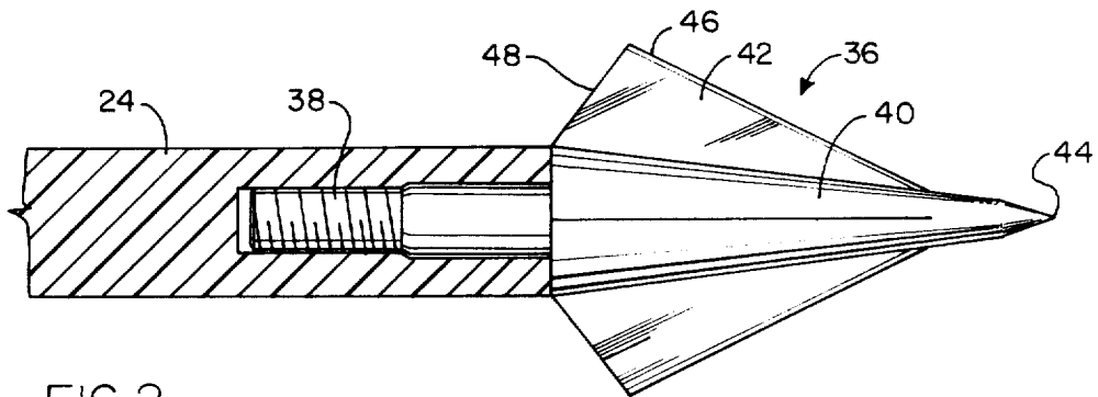
FIG. 2 KNOWN ART
