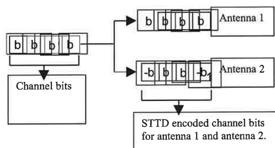
Figure 7: Generic block diagram of the STTD encoder
