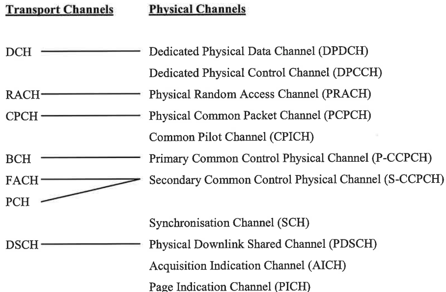
Figure 21: Transport-channel to physical-channel mapping
