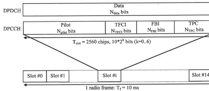
Figure 1: Frame structure for uplink DPDCH/DPCCH
