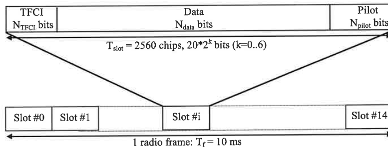
Figure 15: Frame structure for Secondary Common Control Physical Channel
