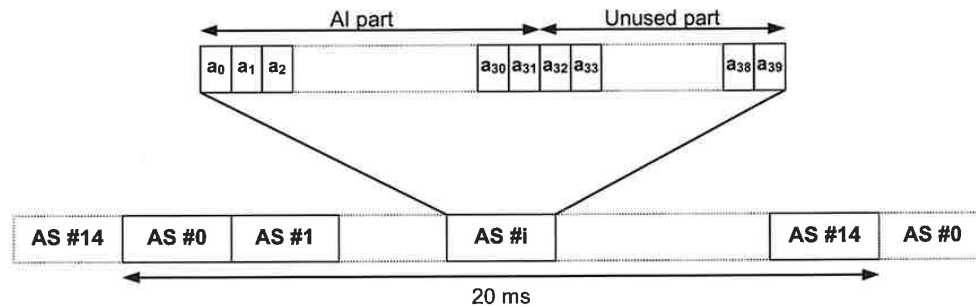
Figure 19: Structure of Acquisition Indicator Channel (AICH)
