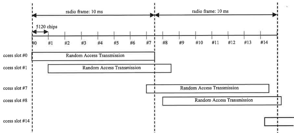
Figure 3: RACH access slot numbers and their spacing
