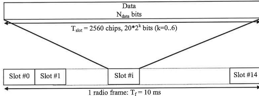
Figure 18: Frame structure for the PDSCH
