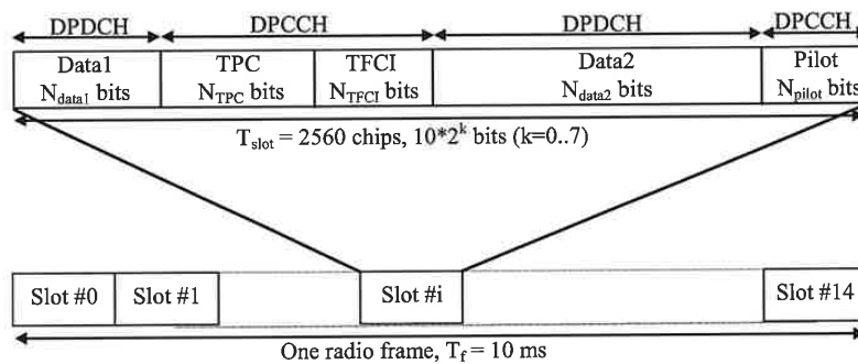
Figure 8: Frame structure for downlink DPCH
