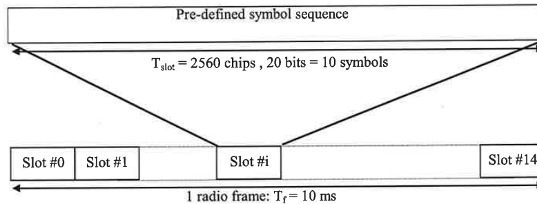
Figure 11: Frame structure for Common Pilot Channel
