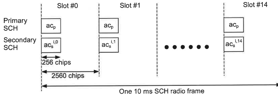
Figure 16: Structure of Synchronisation Channel (SCH)
