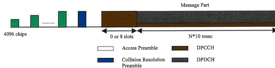
Figure 6: Structure of the CPCH random access transmission
