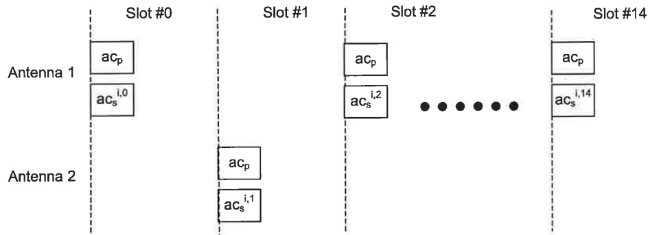
Figure 17: Structure of SCH transmitted by TSTD scheme
