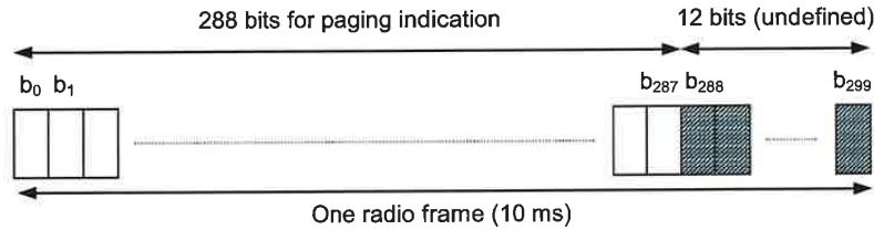
Figure 20: Structure of Page Indicator Channel (PICH)
