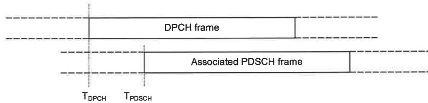
Figure 26: Timing relation between DPCH frame and associated PDSCH frame
