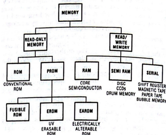
Memory types.
