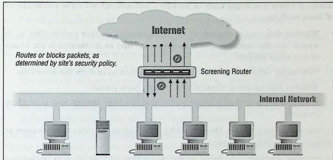
Figure 5-1. Using a screening router to do packet filtering
