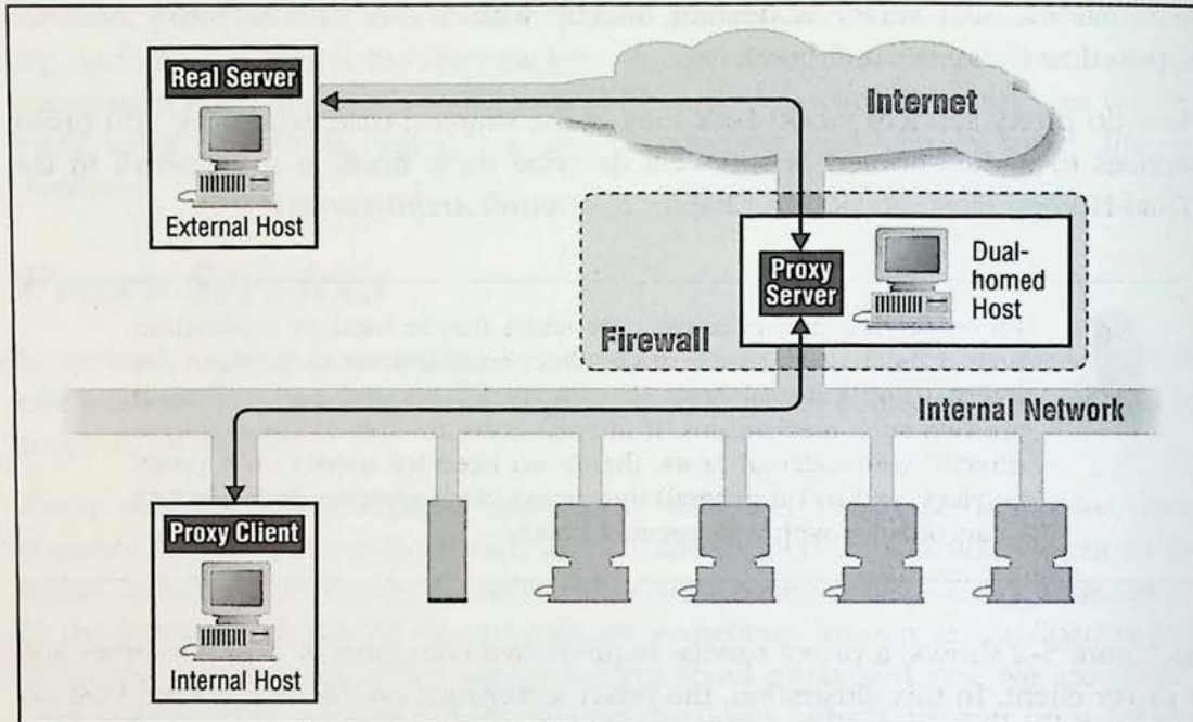
Figure 5-2. Using proxy services with a dual-homed host
