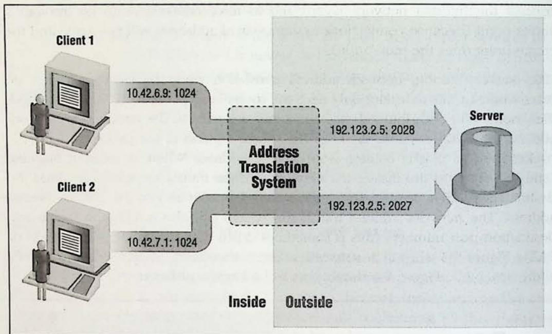
Figure 5-4. Port and address translation
