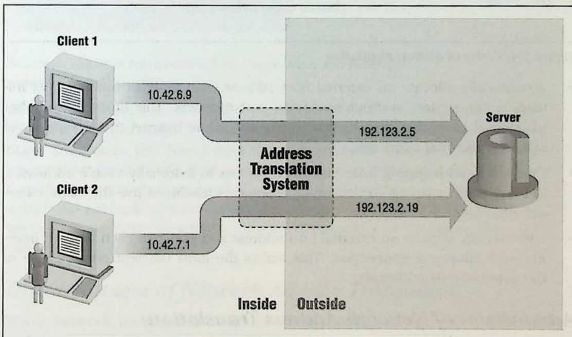
Figure 5-3. Network address translation
