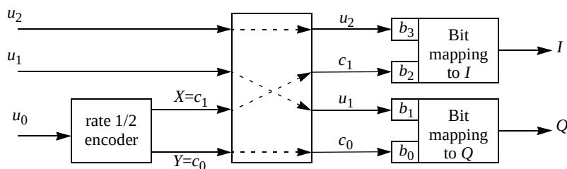
Figure 163—Pragmatic TCM encoder for rate 3/4 16-QAM
