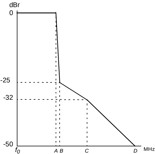
Figure 265—Transmit spectral mask (see Table 341)
