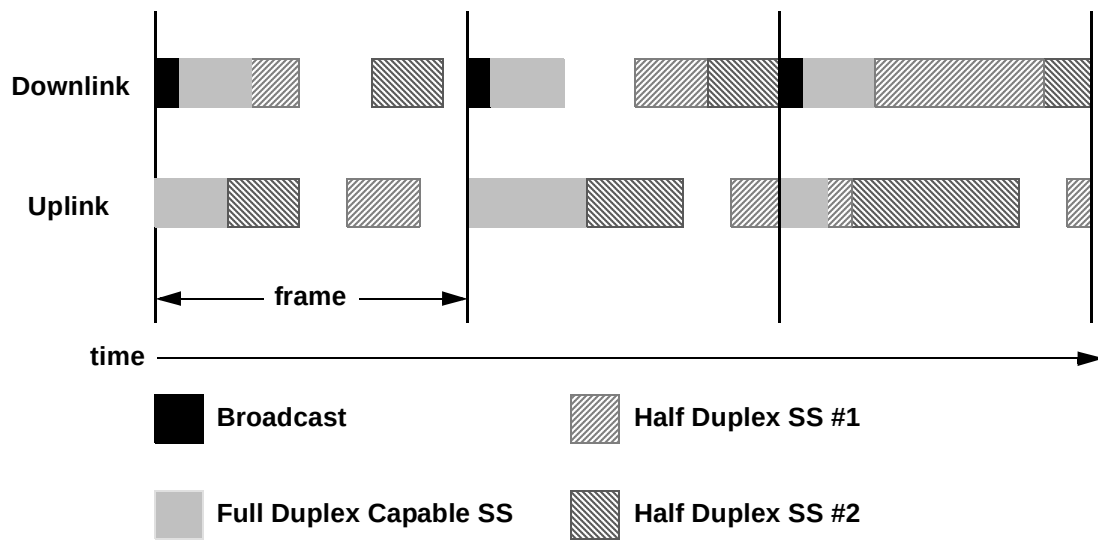
Figure 44—Example of Burst FDD bandwidth allocation
