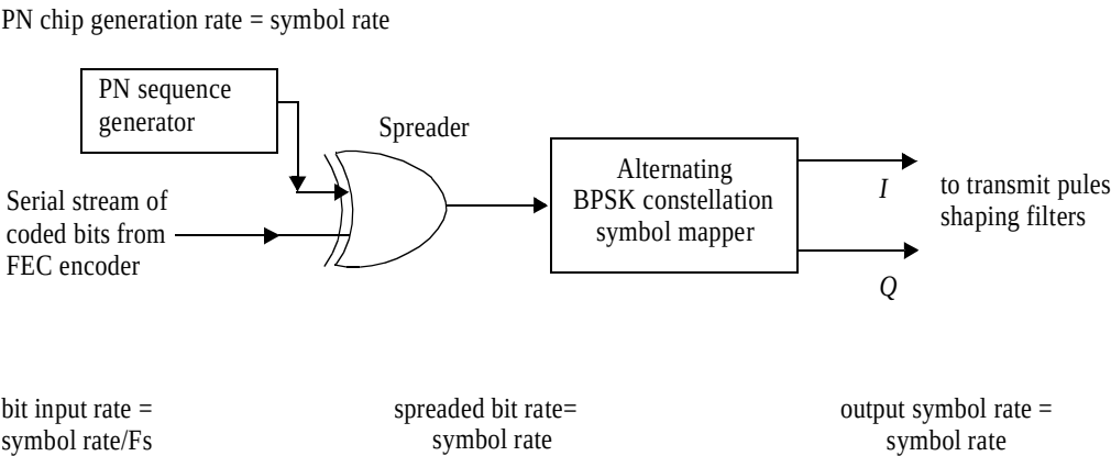
Figure 176—Spread BPSK processing
