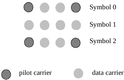
Figure 236—Description of an uplink tile
