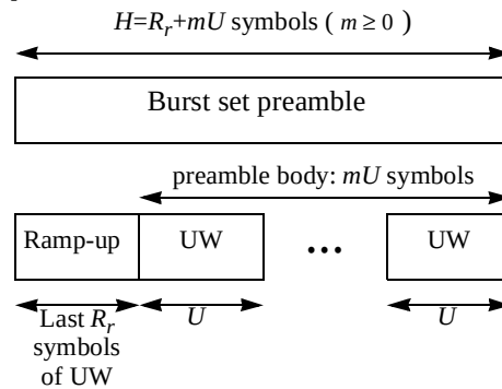
Figure 179—Burst set preamble composition
