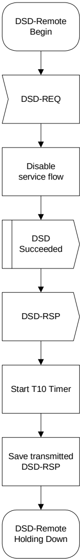
Figure 127—DSD—Remotely Initiated Transaction Begin state flow diagram
