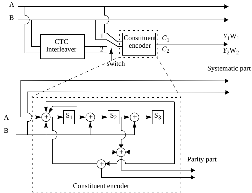
Figure 257—CTC encoder
