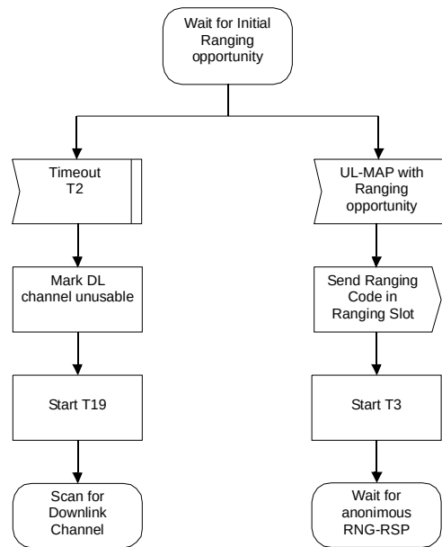
Figure 85—CDMA Initial Ranging—SS (part 1)
