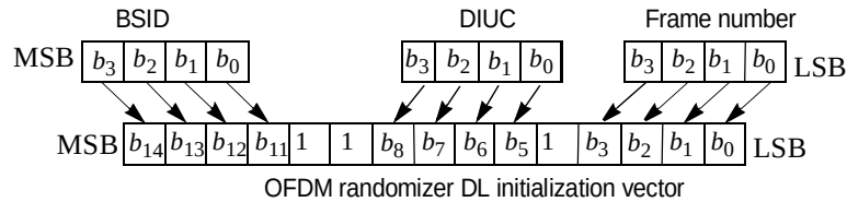
Figure 198—OFDM randomizer downlink initialization vector for burst #2...N
