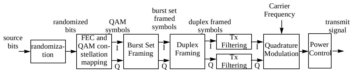
Figure 158—Transmit processing
