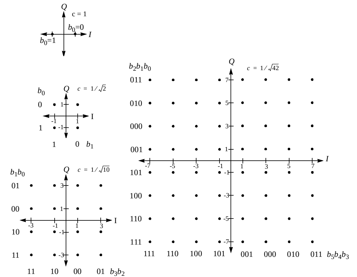
Figure 203—BPSK, QPSK, 16-QAM, and 64-QAM constellations
