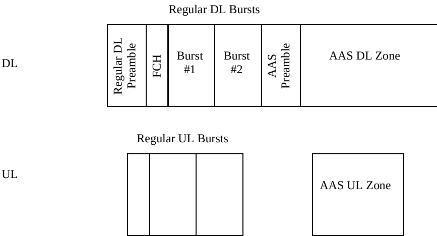
Figure 52—AAS Zone, FDD
