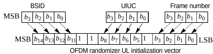
Figure 199—OFDM randomizer uplink initialization vector
