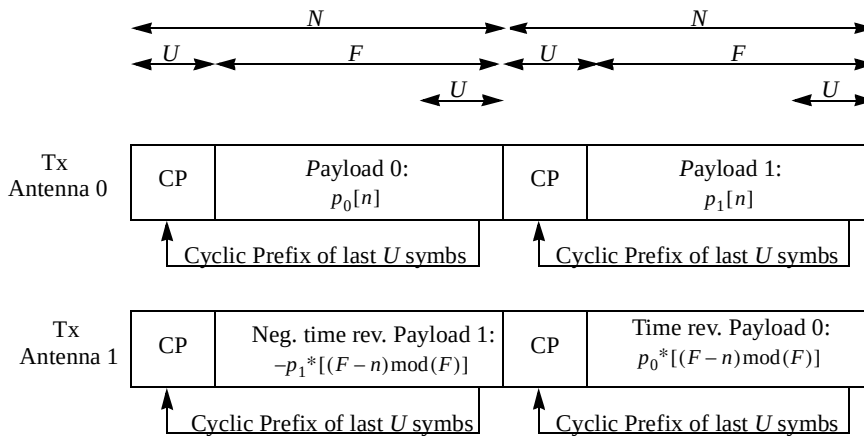
Figure 182—STC dual blocks without UWs
