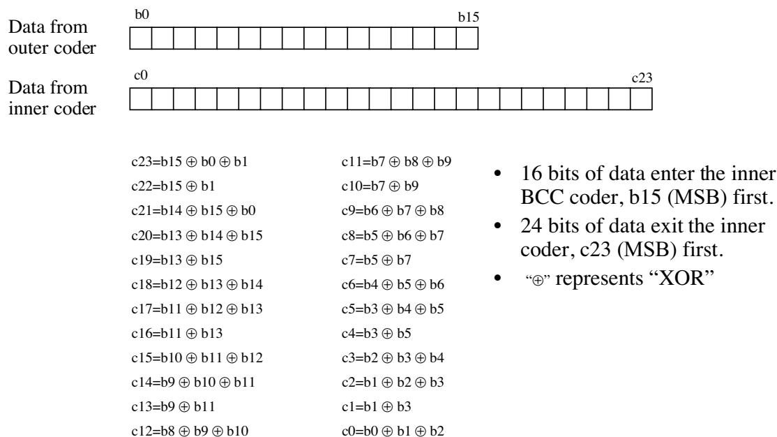
Figure 147—Inner code for Code Type 2 in the downlink
