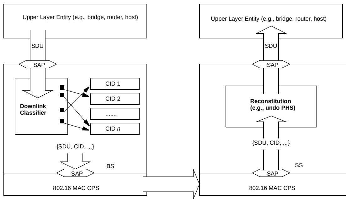
Figure 7—Classification and CID mapping (BS to SS)
