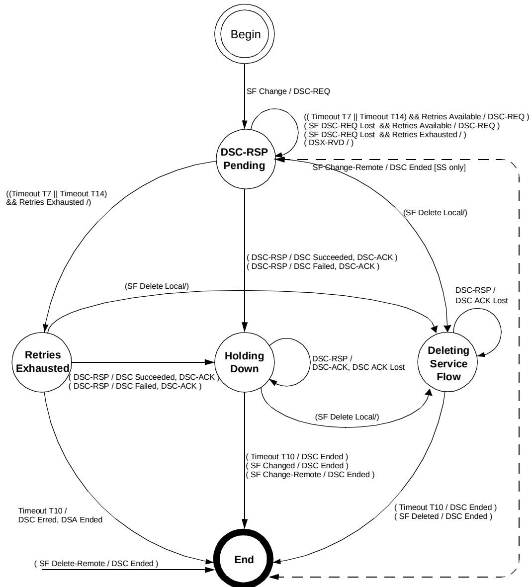
Figure 102—DSC—Locally Initiated Transaction state transition diagram
