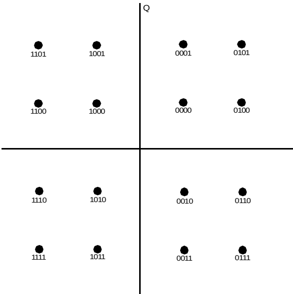
Figure 152—16-QAM constellation (gray-coded)
