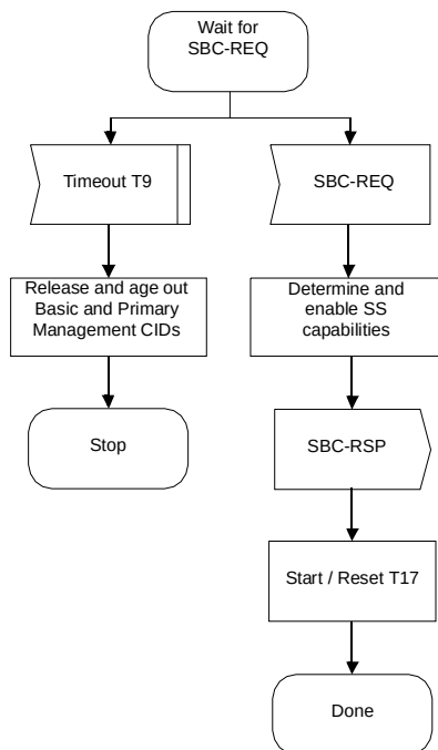
Figure 67—Negotiate Basic Capabilities—BS
