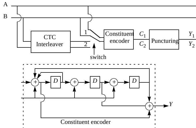
Figure 169—CTC encoder
