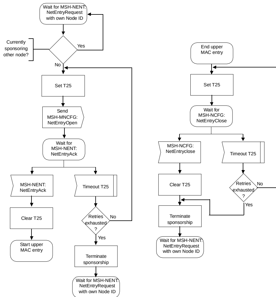
Figure 75—Mesh network synchronization and entry—Sponsor node
