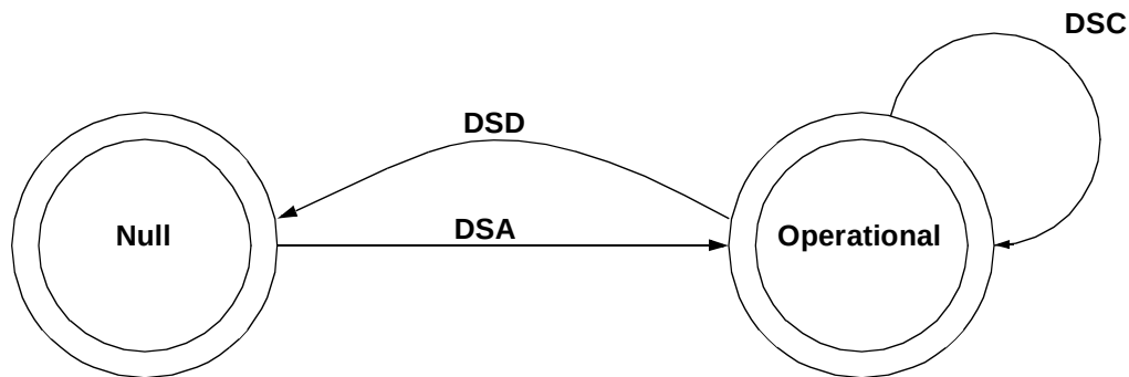
Figure 98—Dynamic service flow overview
