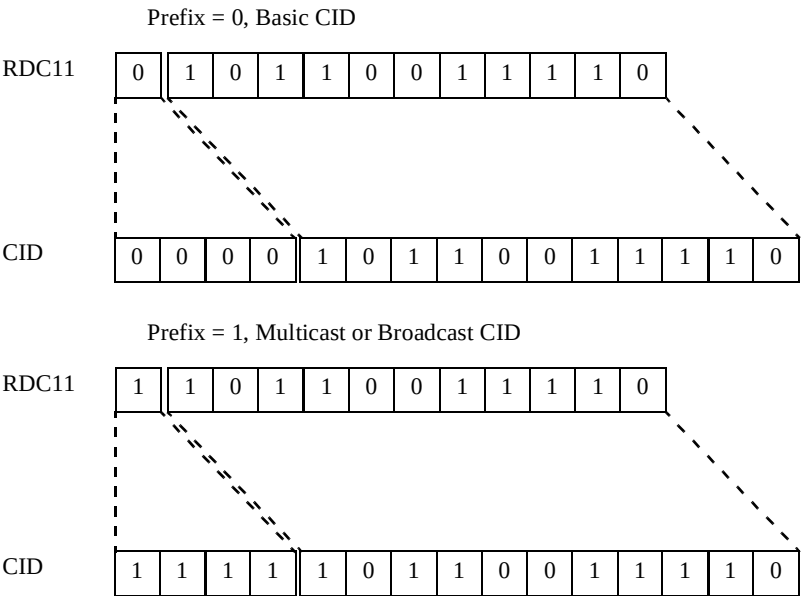
Figure 22—Reduced CID Decoding
