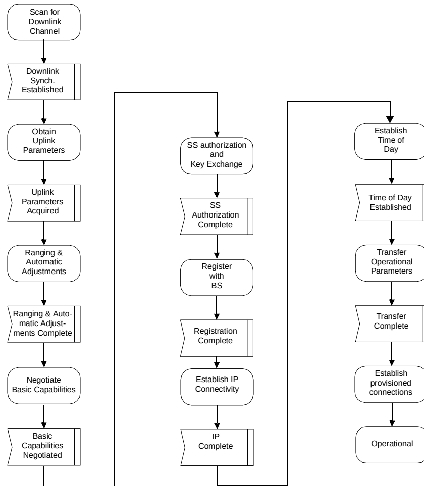
Figure 55—SS Initialization overview
