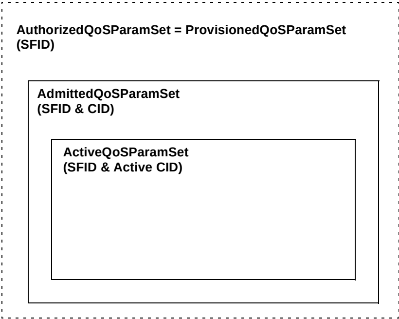
Figure 93—Provisioned authorization model “envelopes”
