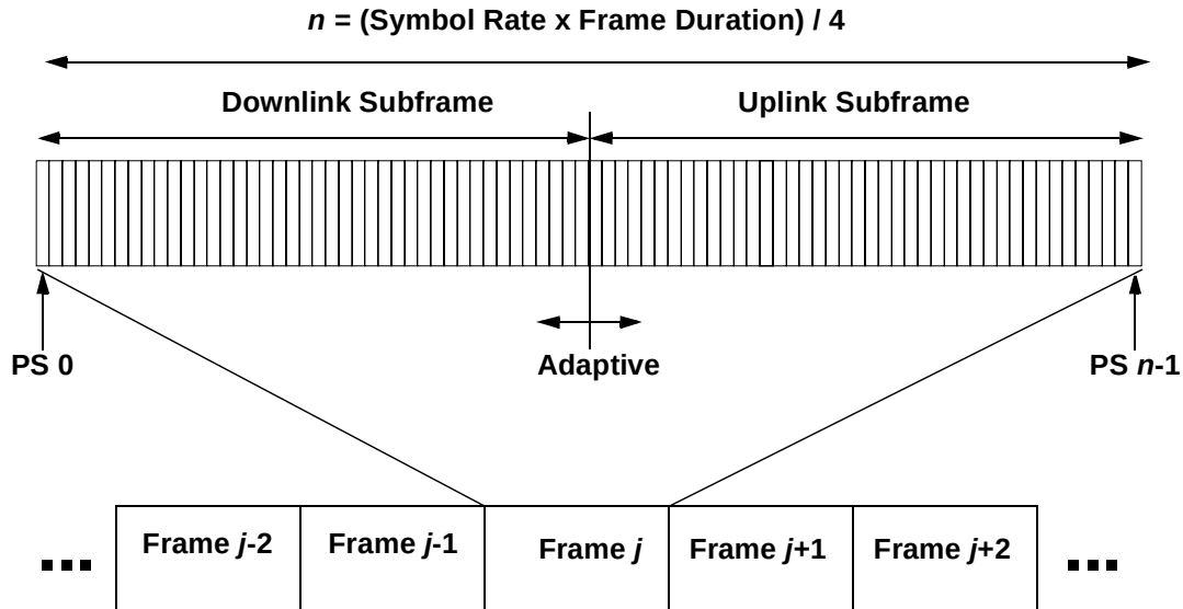
Figure 139—TDD frame structure
