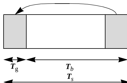
Figure 195—OFDM symbol time structure
