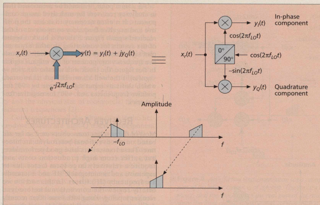
■ Figure 2. Mixing a real signal with a complex exponential. The spectra of the real and complex inputs of the mixer, and the spectrum of the complex output of the mixer are shown. Here, complex signals are represented by double lines.
