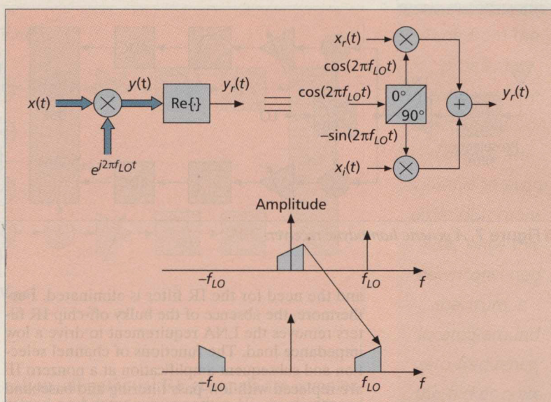
■ Figure 4. An efficient implementation for a complex mixer when only a real part of the mixer output is of interest. The spectra of the complex inputs of the mixer, and the spectrum of the real part of the mixer output are shown. Note that since the final output is real signal, its spectrum is complex-conjugate symmetric.
