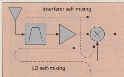
■ Figure 8. Self-mixing of the LO and/or of an interferer in homodyne receiver front-end.
