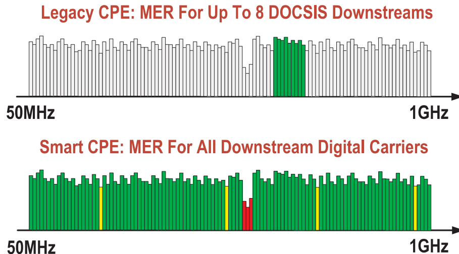
Figure 4. MER coverage of legacy CPE vs Smart CPE
