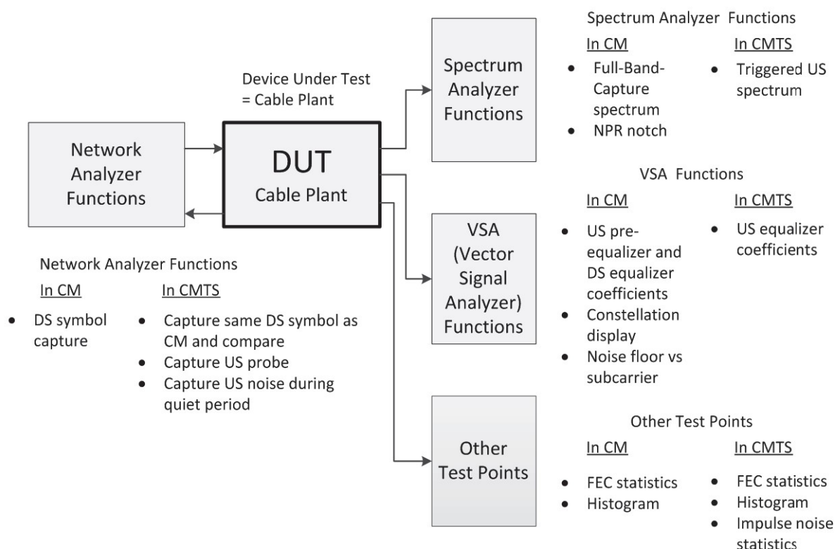
Figure 7. Smart CPE and CMTS can provide essential functions of a network analyzer, spectrum analyzer and VSA to troubleshoot the cable plant.
