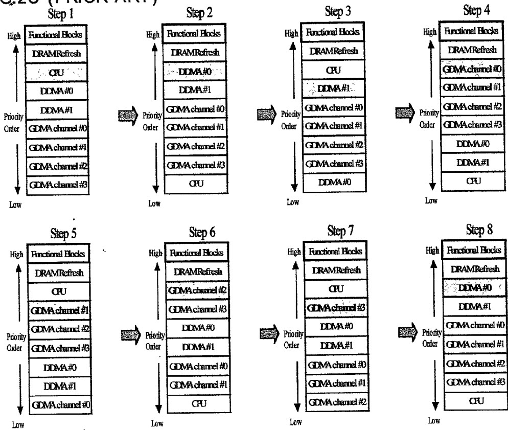
FIG.2C (PRIOR ART)
