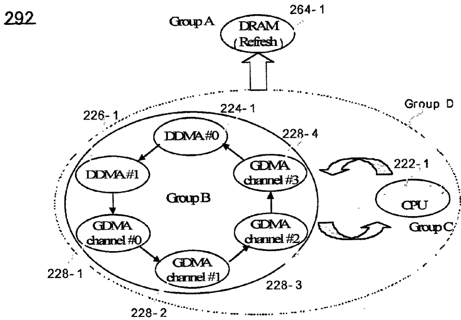
FIG.2C (PRIOR ART)
