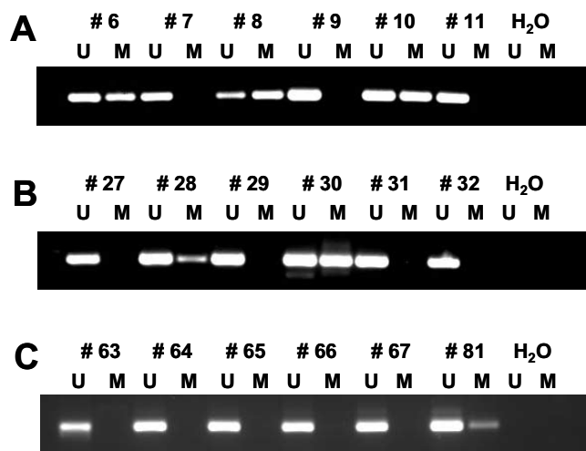
Figure 2. Detection of unmethylated (u) and methylated (m) HIC1 promoter DNA in stool samples from patients with (A) CRC, (B) adenoma, and (C) normal controls.
