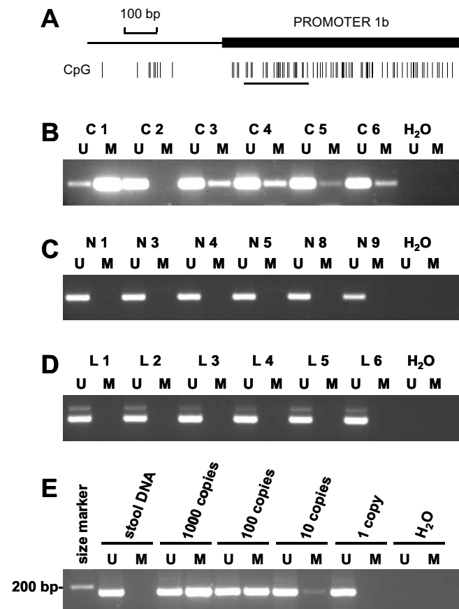
Figure 1. (A) Location of the amplified region (underlined) of the HIC1 promoter by MSP. (B) Detection of unmethylated (u) and methylated (m) HIC1 promoter DNA in primary CRCs, (C) normal colonic epithelium, and (D) human peripheral blood leukocytes. (E) Analysis of sensitivity of the HIC1 MSP assay. Indicated genome equivalents of fully methylated DNA were spiked into normal stool DNA.
