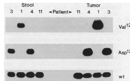
Fig. 2. Southern blot assay for ras mutations. PCR products that contained the first coding exon of K-ras were generated from stools and tumors of patients 1, 3, 4, and 11, as indicated (16). PCR products were subjected to electrophoresis through a 2% agarose gel and transferred to nylon filters (21). The blots were hybridized to oligonucleotide probes specific for wild-type ras (bottom), the Asp 12 mutation (middle), or the Val 12 mutation (top).
