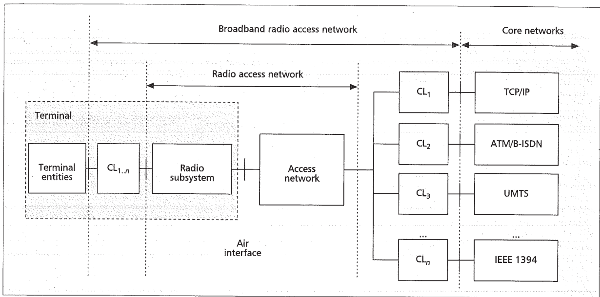
■ Figure 1. The HIPERLAN/2 reference model [2].
