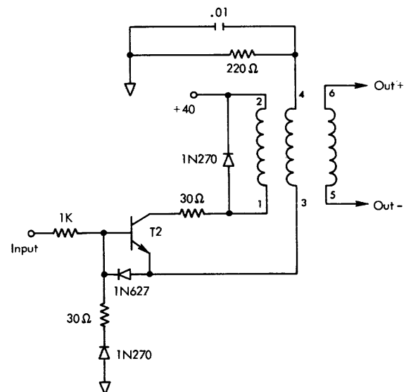
Figure 9. Blocking Oscillator.
