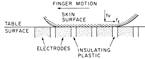
Fig. 6. Applicable forces.
