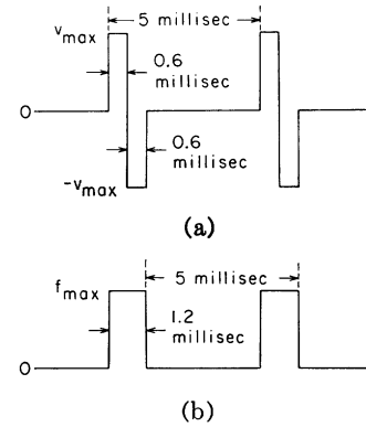
Fig. 8. Voltage and pulse waveforms.
