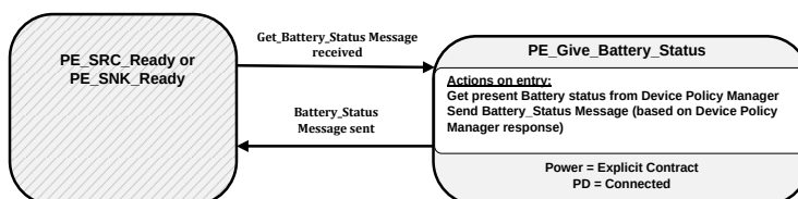
Figure 8-76 Give Battery Status state diagram
