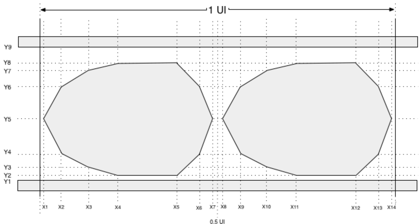
Figure 5-15 BMC Tx 'ONE' Mask
