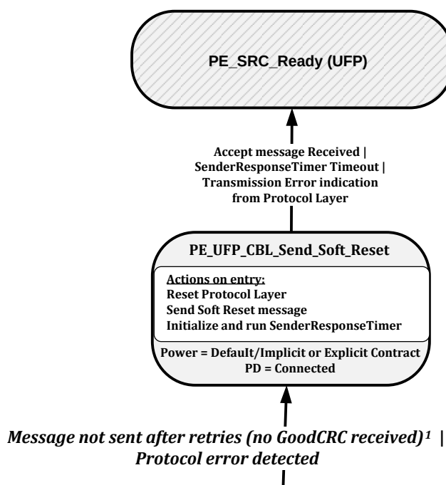
Figure 8-114 UFP Source Soft Reset of a Cable Plug State Diagram
