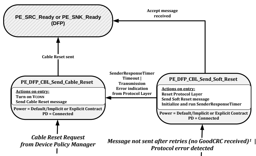
Figure 8-113 DFP Soft Reset or Cable Reset of a Cable Plug State Diagram
