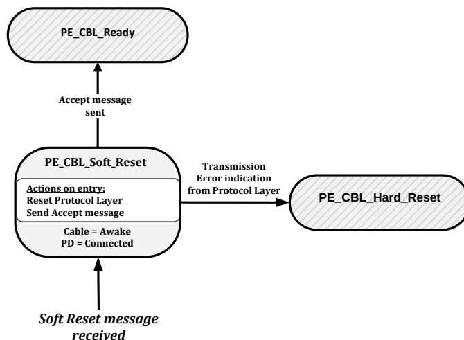
Figure 8-111 Cable Plug Soft Reset State Diagram
