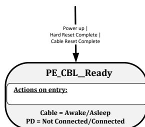
Figure 8-110 Cable Ready VDM State Diagram
