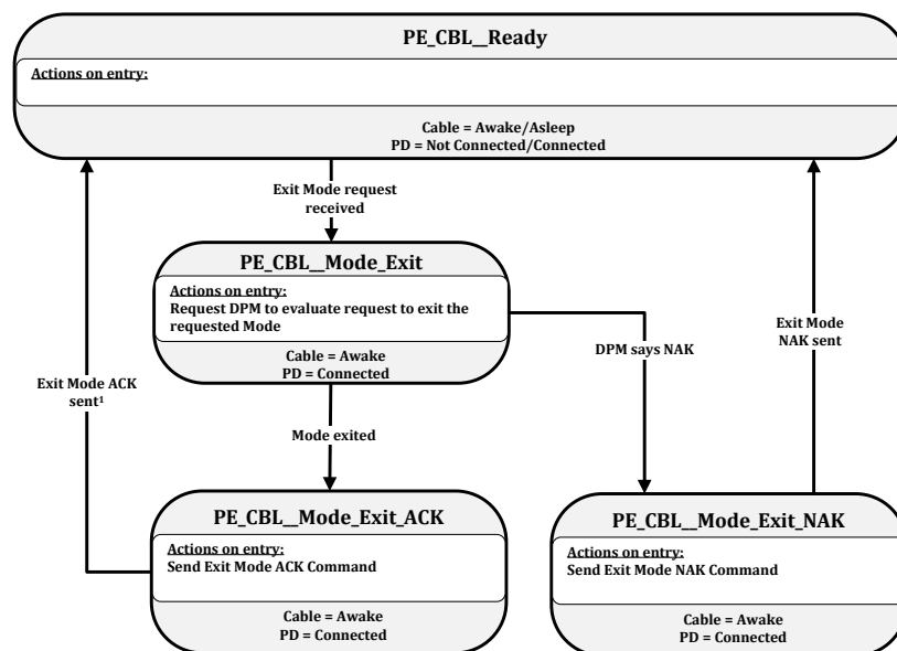
Figure 8-117 Cable Plug Structured VDM Exit Mode State Diagram
