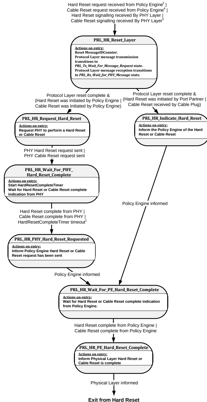
Figure 6-46 Hard/Cable Reset
