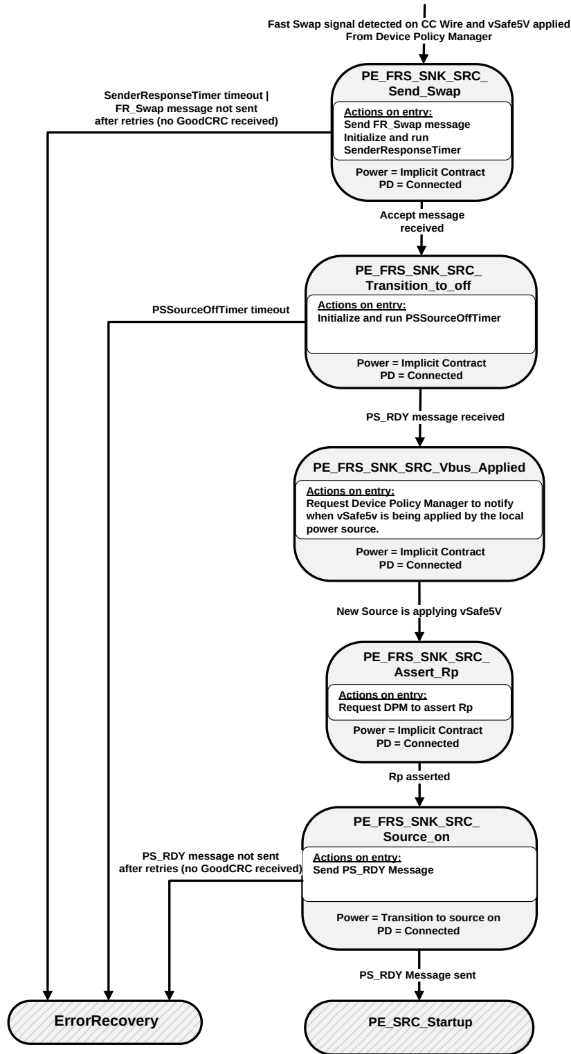
Figure 8-90: Dual-role Port in Sink to Source Fast Role Swap State Diagram
