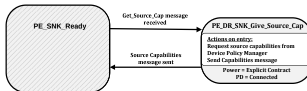
Figure 8-94 Dual-Role (Sink) Give Source Capabilities State Diagram
