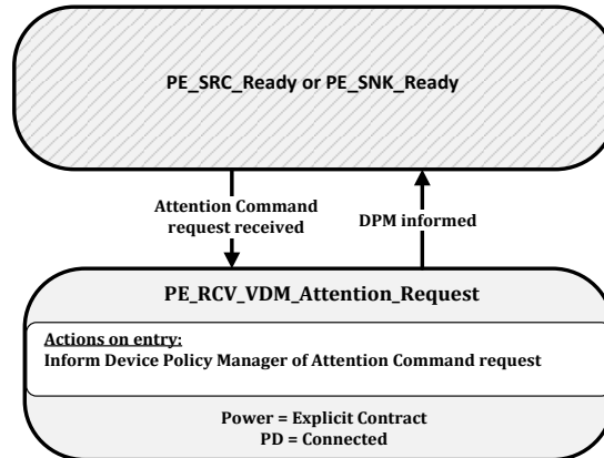
Figure 8-105 Receiving a Structured VDM Attention State Diagram
