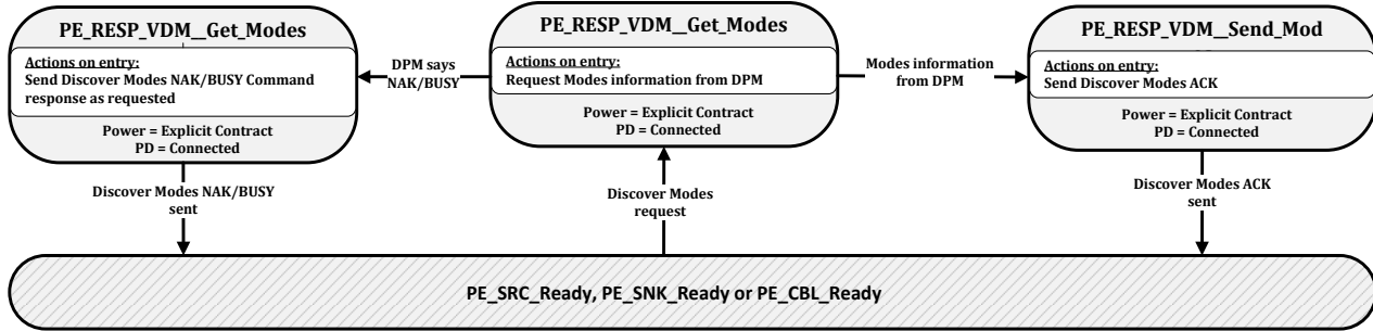
Figure 8-104 Responder Structured VDM Discover Modes State Diagram
