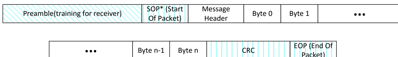
Figure 5-3 USB Power Delivery Packet Format
