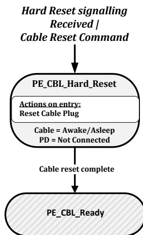
Figure 8-112 Cable Plug Hard Reset State Diagram
