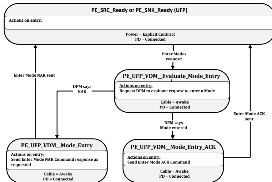
Figure 8-108 UFP Structured VDM Enter Mode State Diagram
