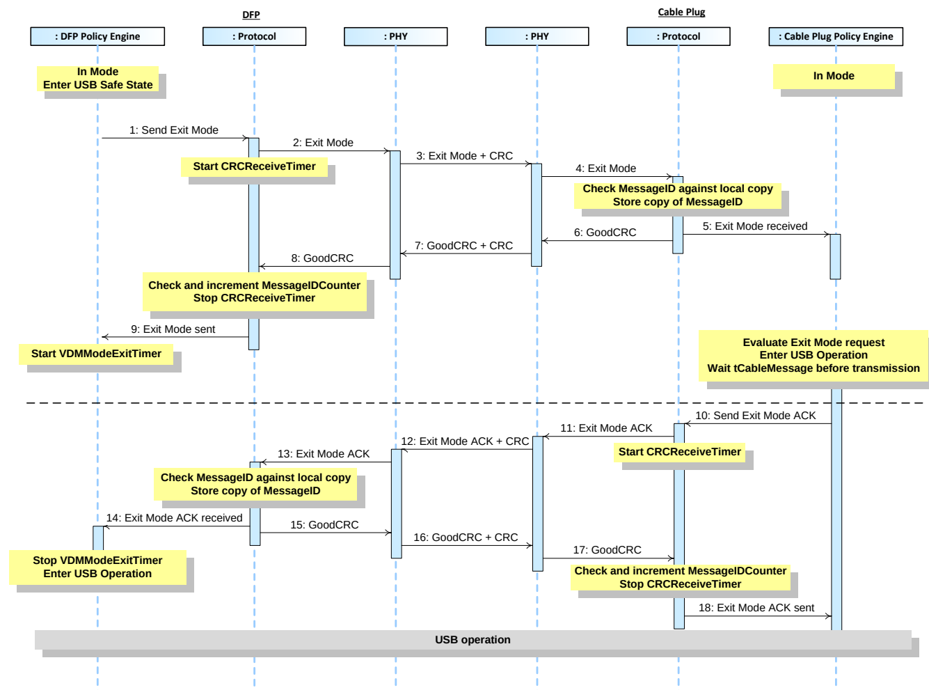
Figure 8-49 DFP to Cable Plug Exit Mode
