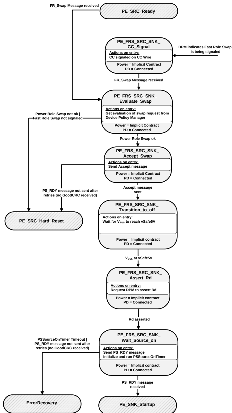
Figure 8-89: Dual-Role Port in Source to Sink Fast Role Swap State Diagram
