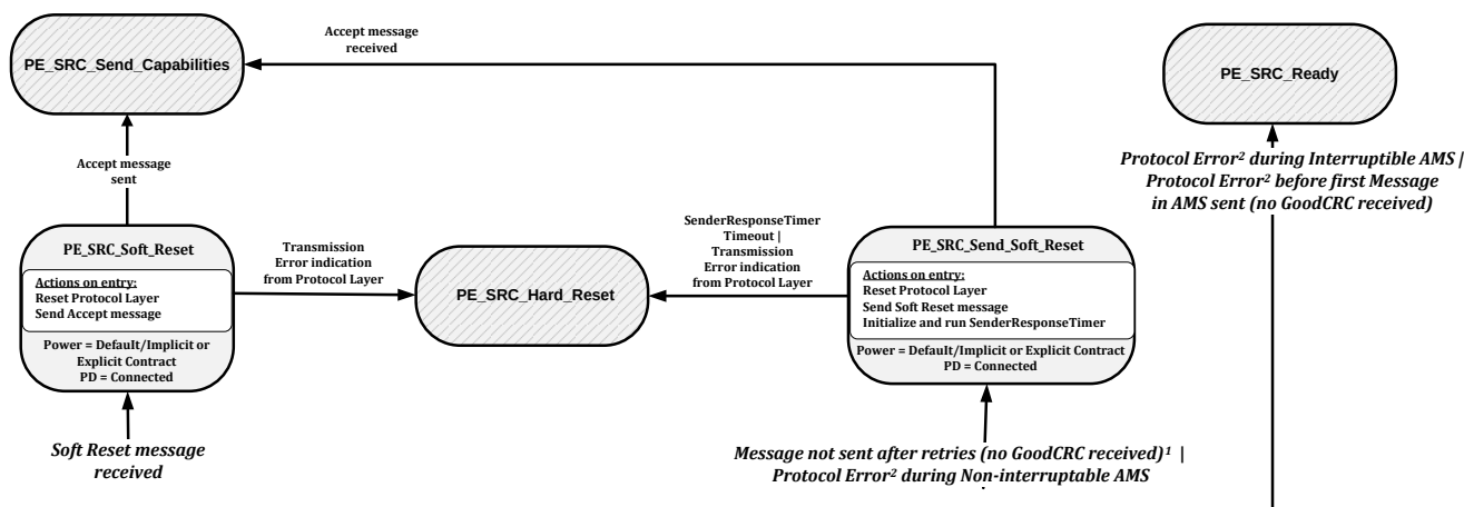
Figure 8-58 Source Port Soft Reset and Protocol Error State Diagram
