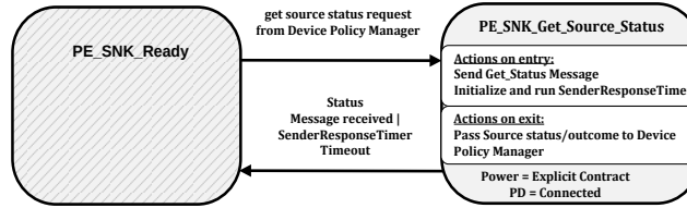
Figure 8-69 Sink Port Get Source Status state diagram
