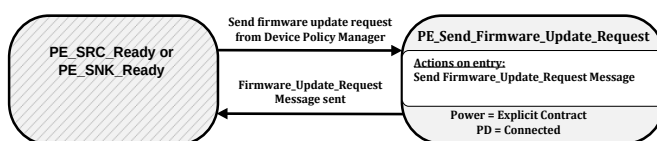
Figure 8-82 Send firmware update request state diagram
