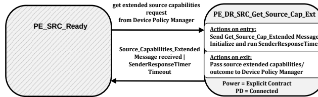
Figure 8-95 Dual-Role (Source) Get Source Capabilities Extended state diagram
