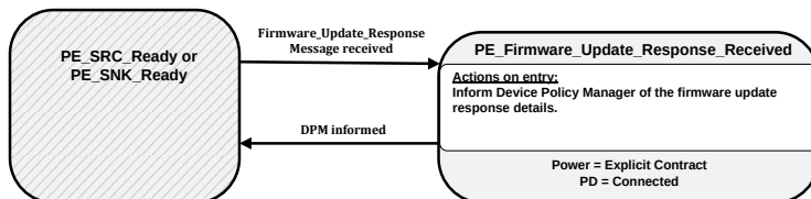
Figure 8-84 Firmware update response received state diagram
