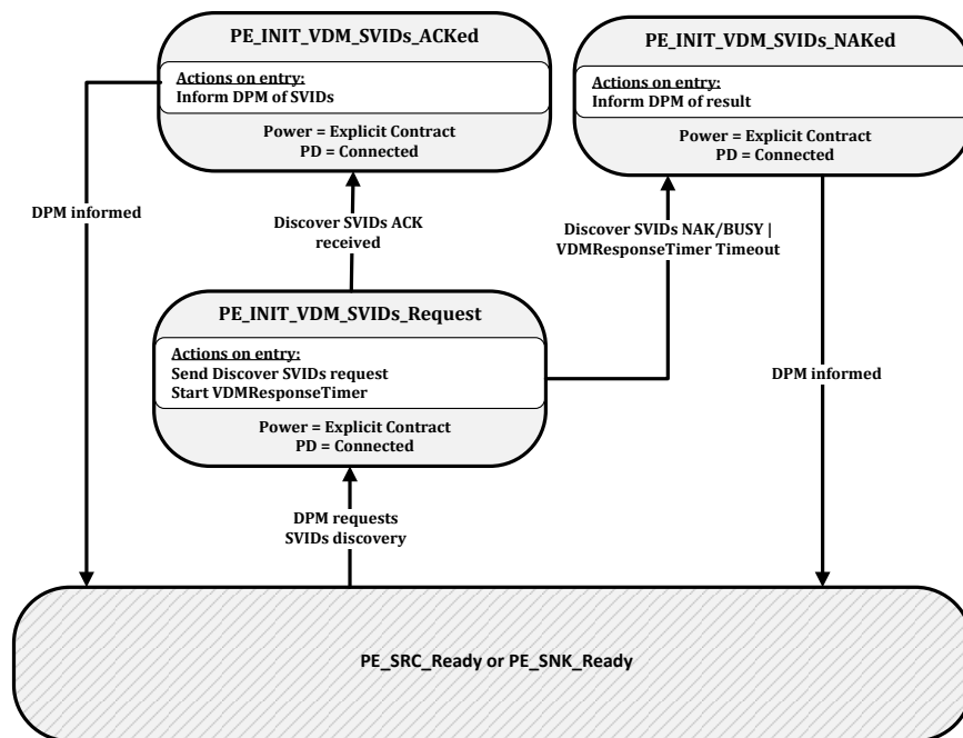
Figure 8-99 Initiator VDM Discover SVIDs State Diagram
