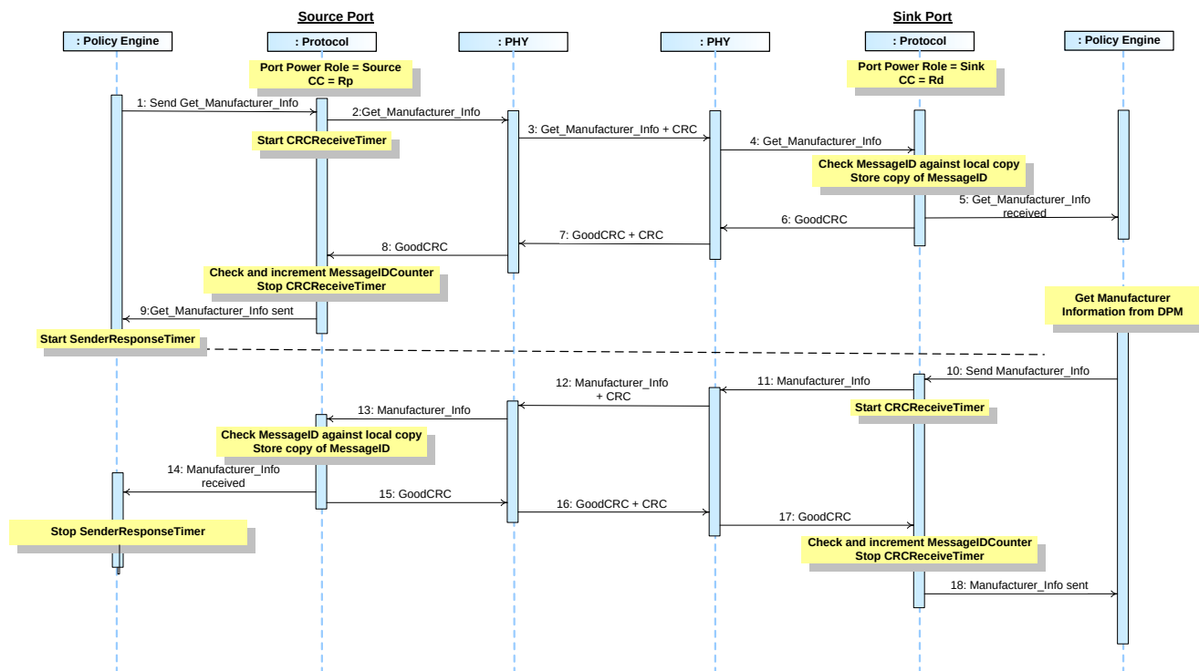
Figure 8-32 Source Gets Sink's Port Manufacturer Information
