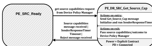
Figure 8-91 Dual-Role (Source) Get Source Capabilities diagram
