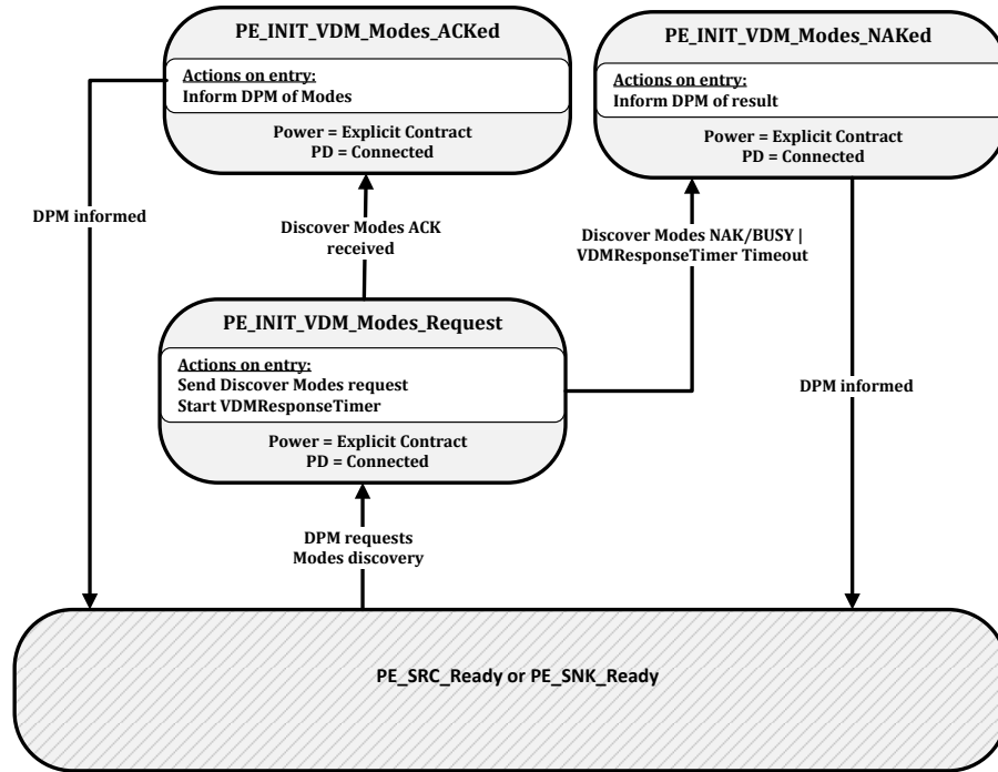
Figure 8-100 Initiator VDM Discover Modes State Diagram
