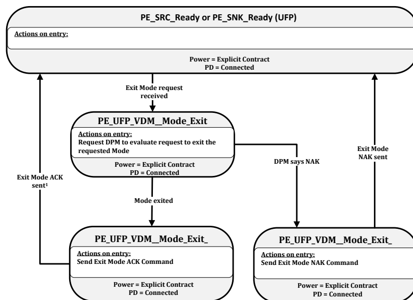
Figure 8-109 UFP Structured VDM Exit Mode State Diagram
