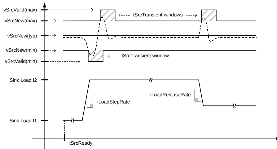
Figure 7-5 Application of v_{SrcNew} and v_{SrcValid} limits after t_{SrcReady}
