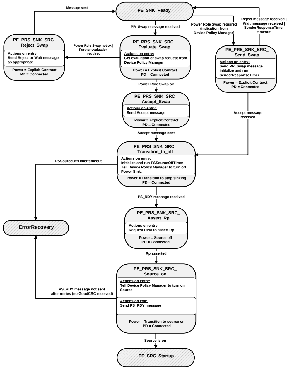
Figure 8-88: Dual-role Port in Sink to Source Power Role Swap State Diagram
