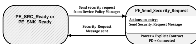
Figure 8-79 Send security request state diagram
