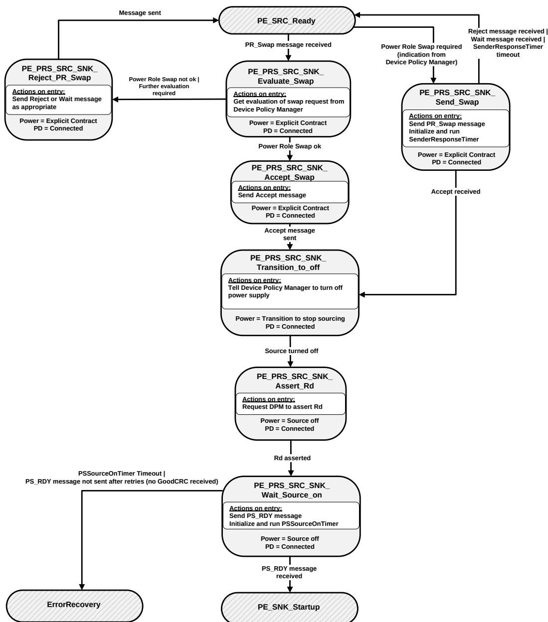
Figure 8-87: Dual-Role Port in Source to Sink Power Role Swap State Diagram
