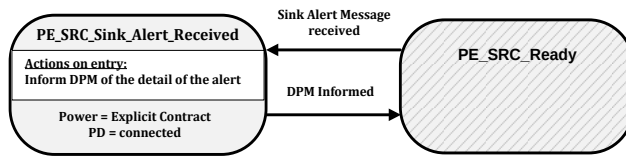
Figure 8-66 Source Port Sink Alert State Diagram
