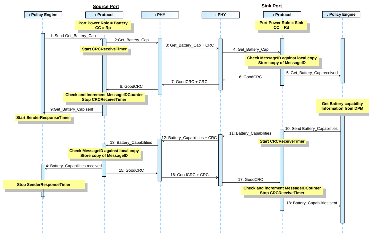
Figure 8-31 Source Gets Sink's Battery Capabilities
