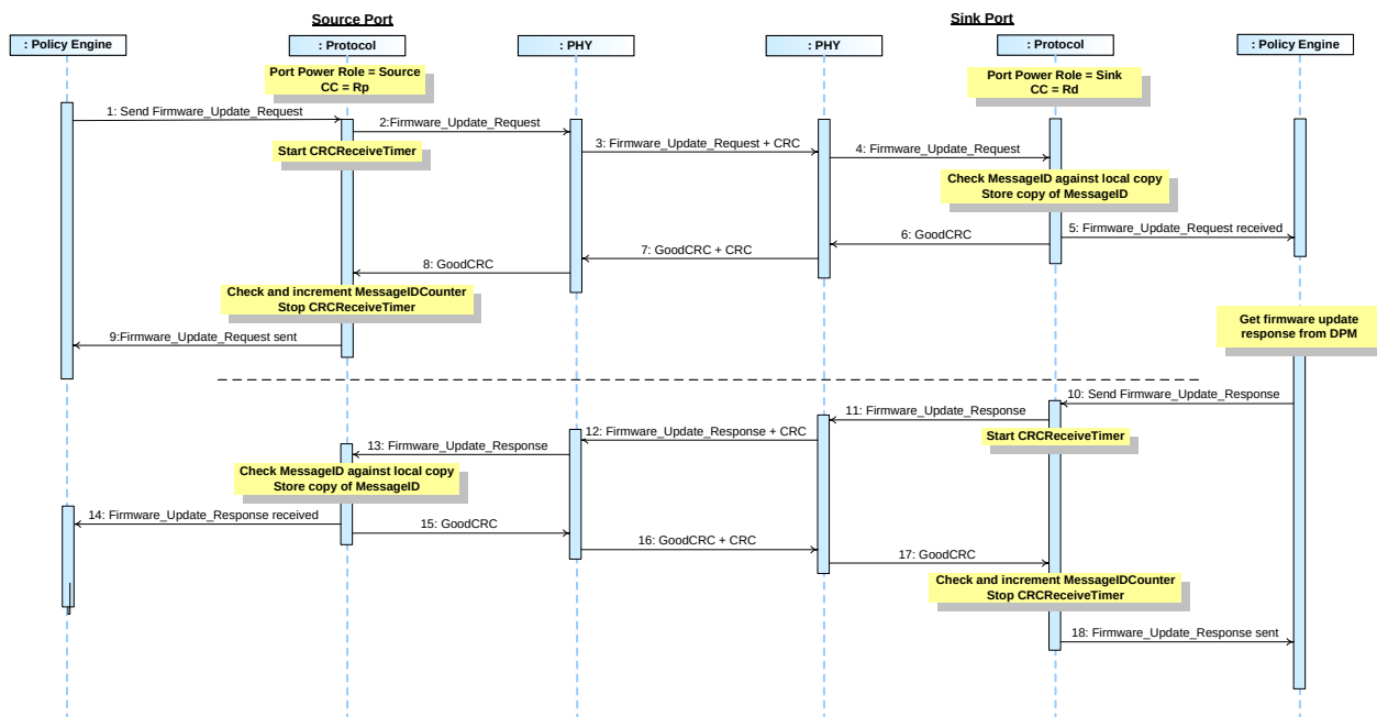
Figure 8-40 Source requests firmware update exchange with Sink
