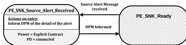
Figure 8-64 Sink Port Source Alert State Diagram
