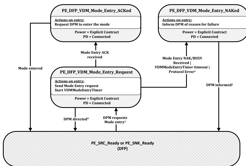
Figure 8-106 DFP VDM Mode Entry State Diagram
