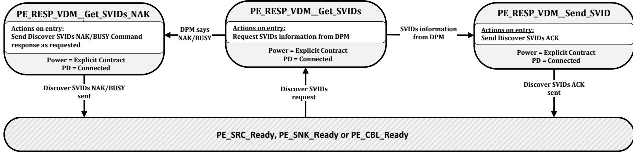
Figure 8-103 Responder Structured VDM Discover SVIDs State Diagram
