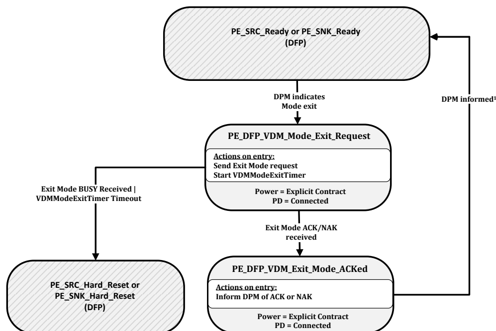
Figure 8-107 DFP VDM Mode Exit State Diagram
