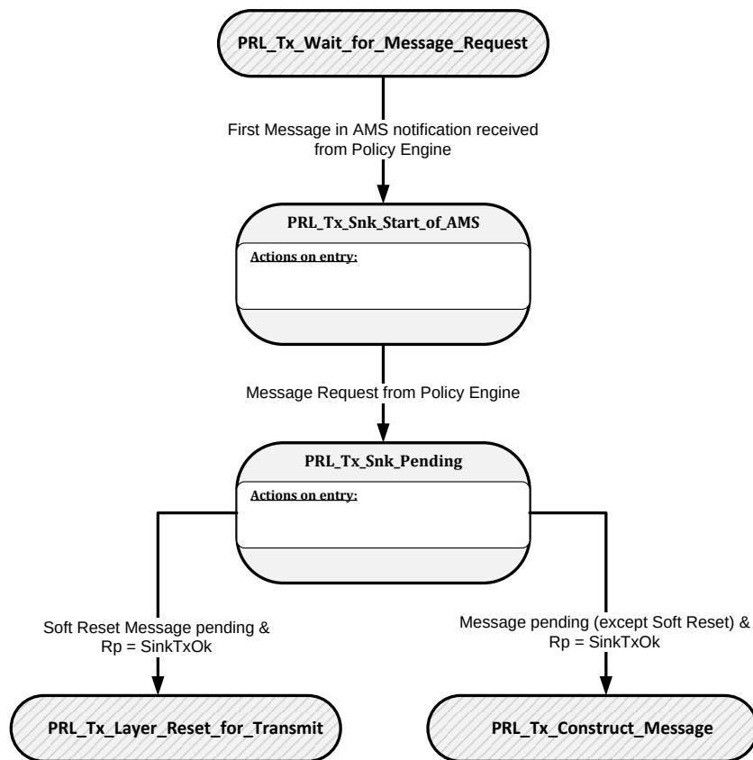
Figure 6-44 Sink Protocol Layer Message transmission State Diagram
