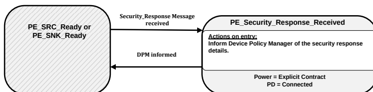
Figure 8-81 Security response received state diagram
