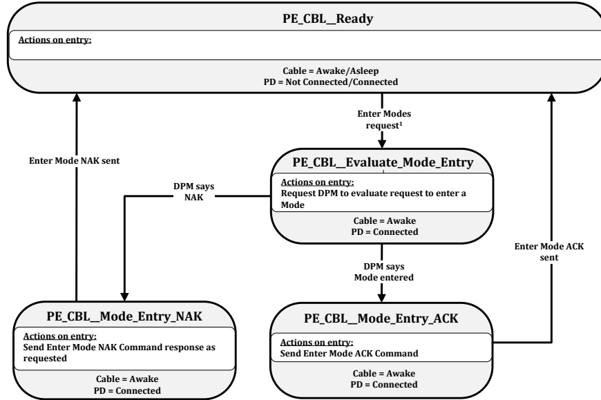
Figure 8-116 Cable Plug Structured VDM Enter Mode State Diagram
