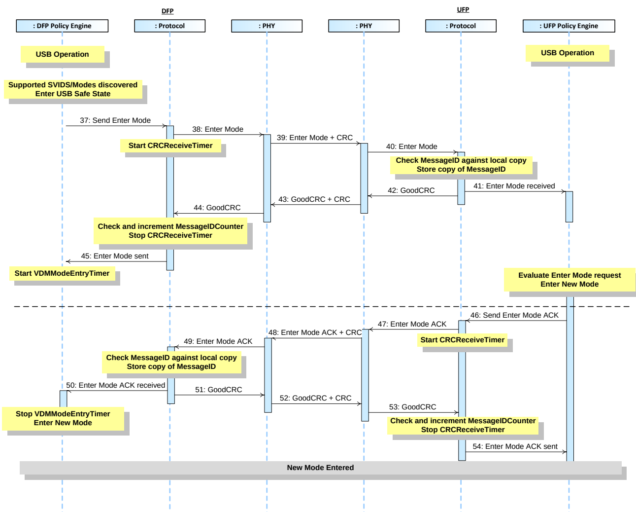
Figure 8-46 DFP to UFP Enter Mode
