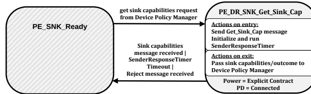
Figure 8-93 Dual-Role (Sink) Get Sink Capabilities State Diagram
