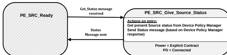
Figure 8-70 Source Give Source Status state diagram
