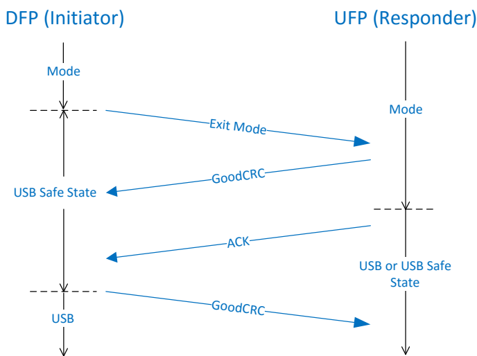
Figure 6-23 Exit Mode sequence
