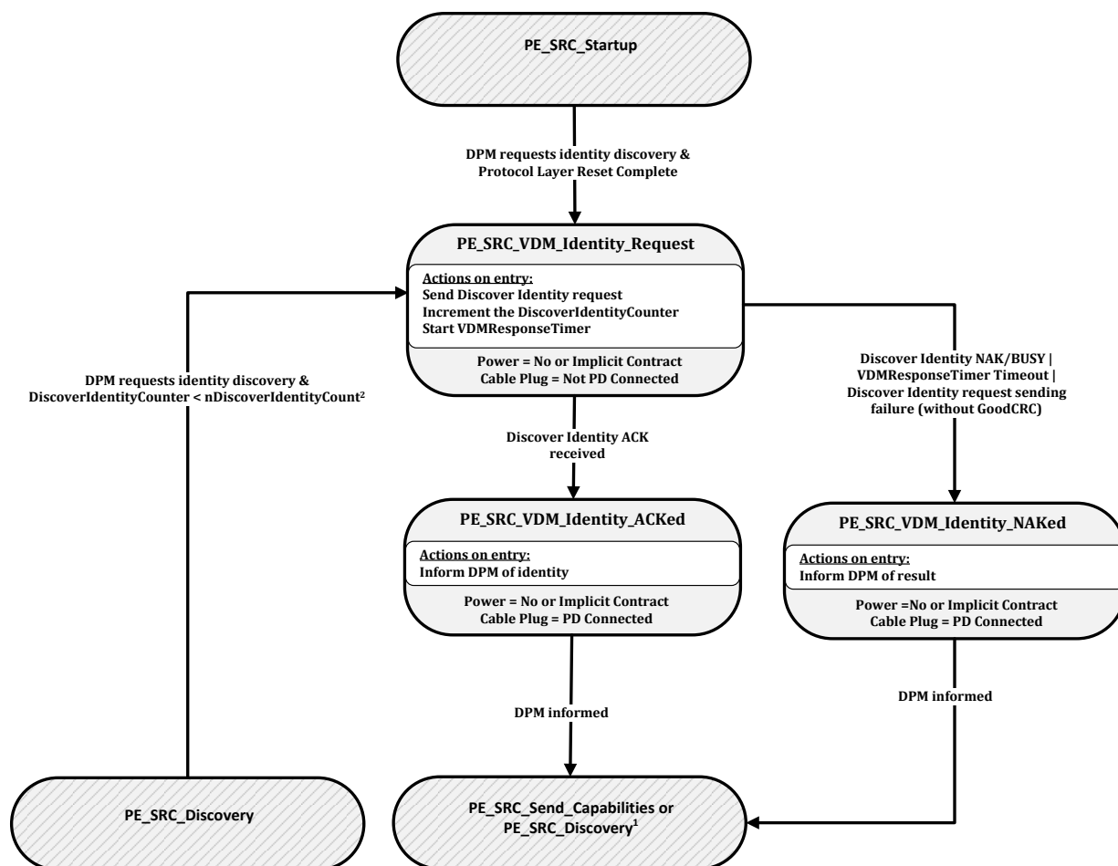
Figure 8-115 Source Startup Structured VDM Discover Identity State Diagram
