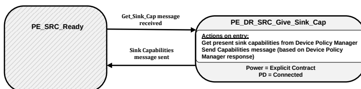
Figure 8-92 Dual-Role (Source) Give Sink Capabilities diagram
