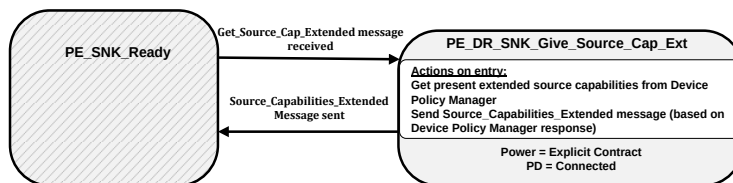
Figure 8-96 Dual-Role (Source) Give Sink Capabilities diagram
