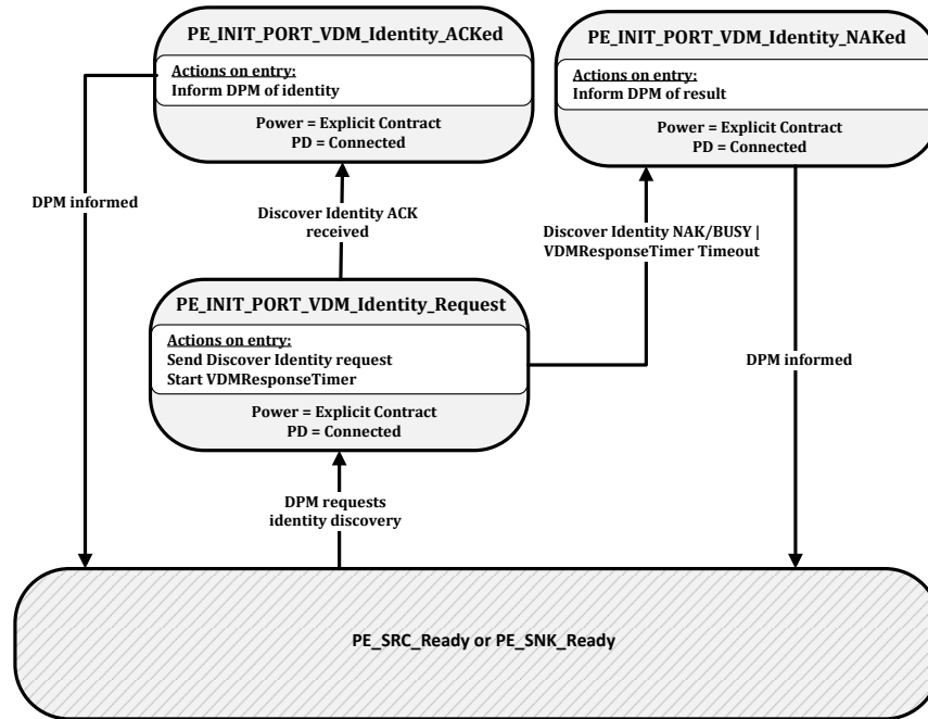
Figure 8-98 Initiator to Port VDM Discover Identity State Diagram
