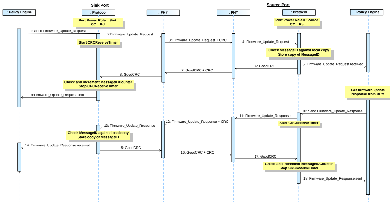
Figure 8-41 Sink requests firmware update exchange with Source
