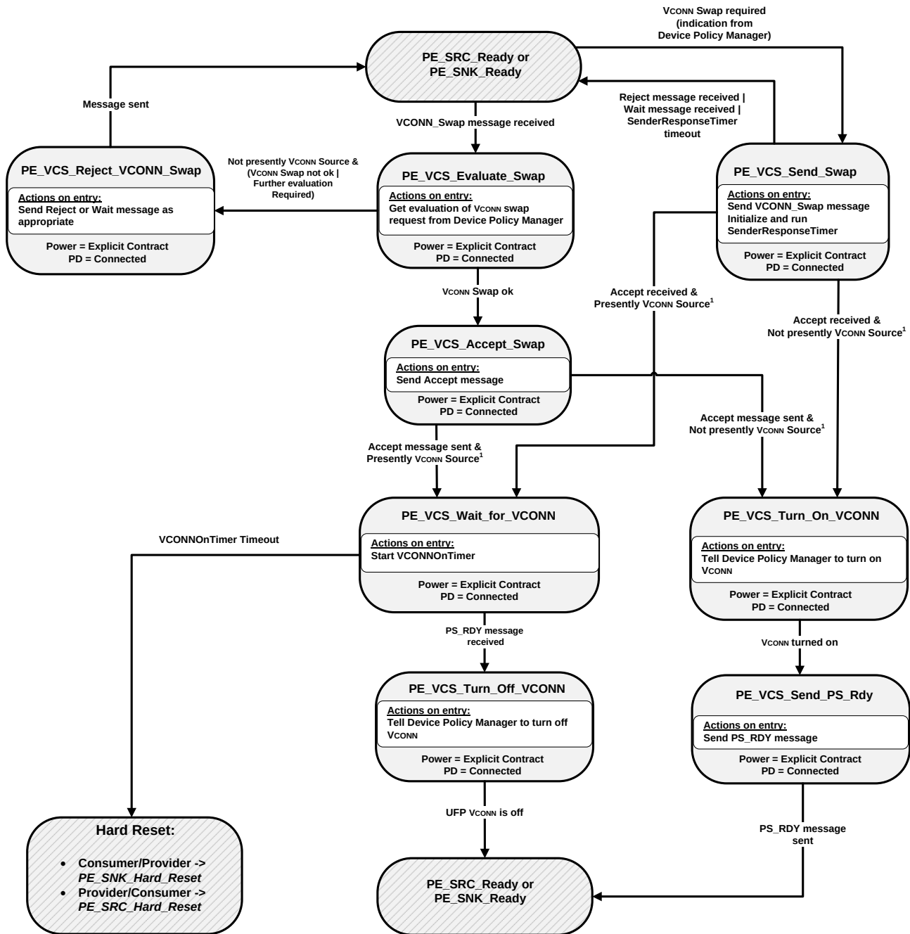
Figure 8-97 VCONN Swap State Diagram
