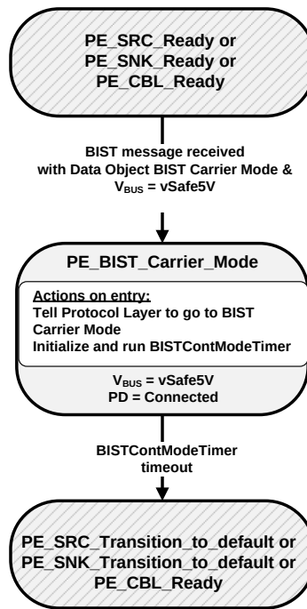
Figure 8-118 BIST Carrier Mode State Diagram
