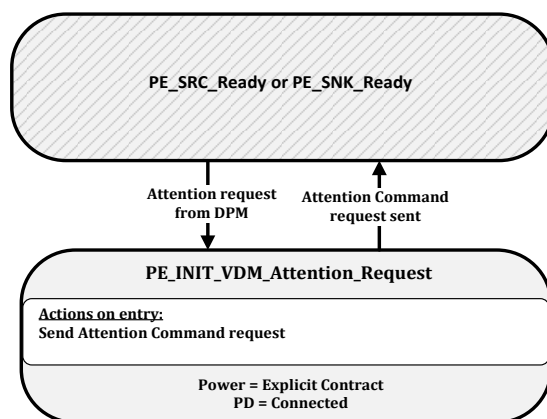
Figure 8-101 Initiator VDM Attention State Diagram
