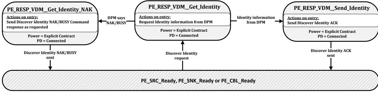
Figure 8-102 Responder Structured VDM Discover Identity State Diagram
