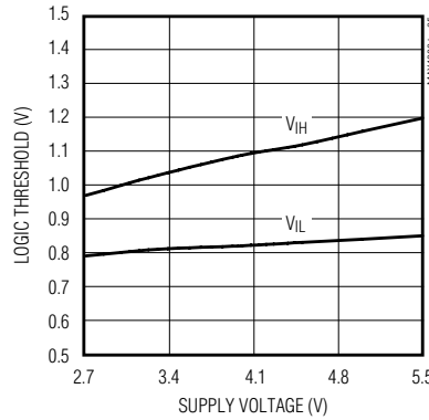
INPUT LOGIC THRESHOLD vs. SUPPLY VOLTAGE
