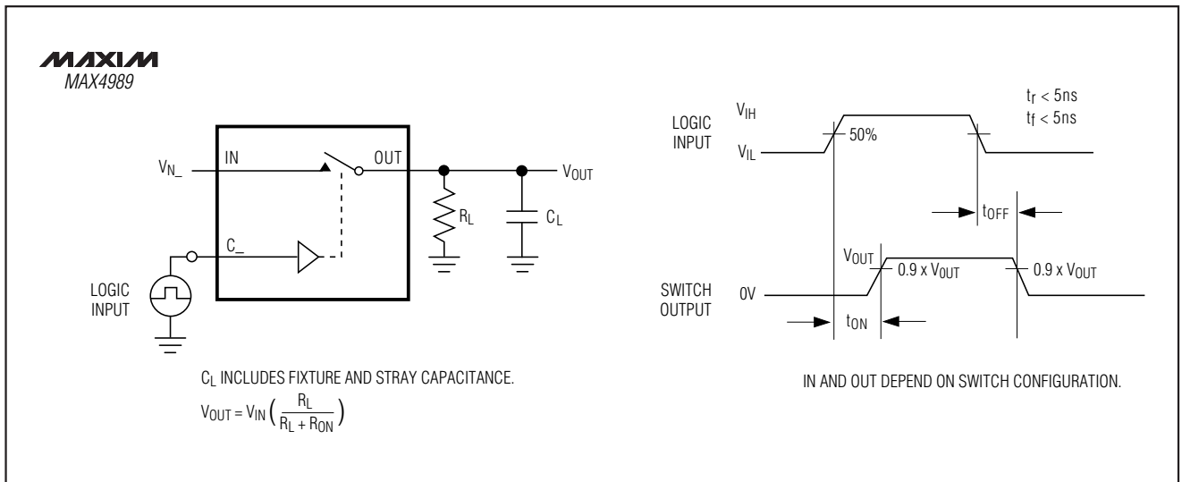
Figure 2. Switching Time
