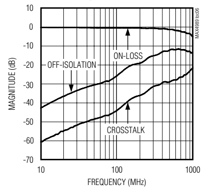
FREQUENCY RESPONSE
