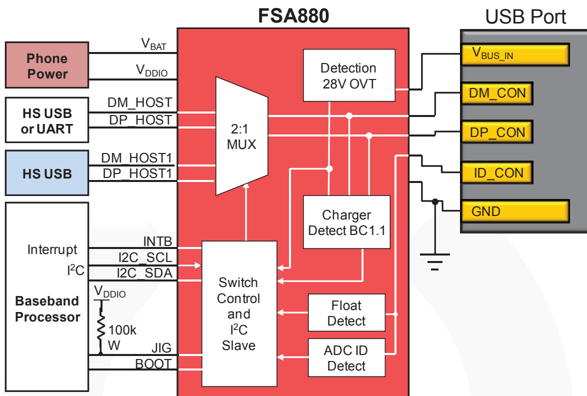
Figure 2. Block Diagram
