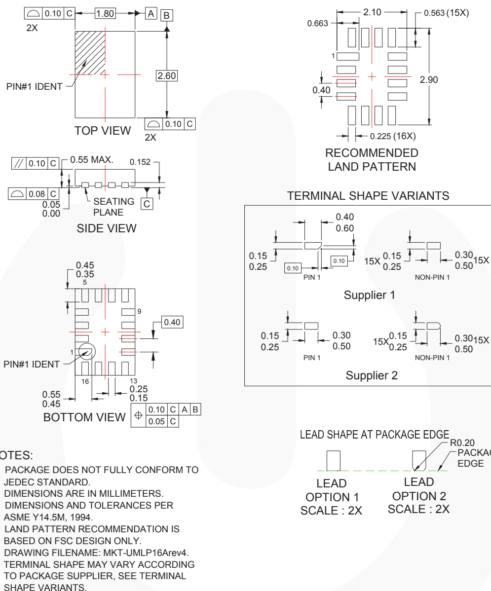
Figure 24. 16-Lead Ultrathin Molded Leadless Package (UMLP), 1.8mm x 2.6mm x 0.55mm, 0.4mm Pitch
