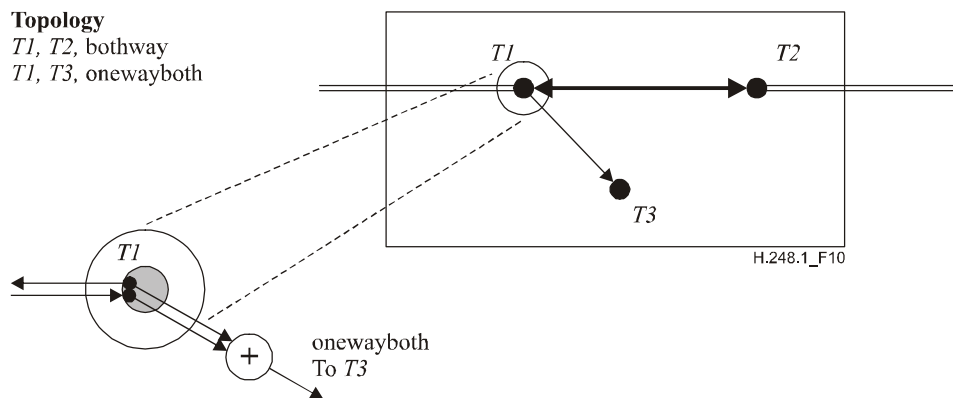
Figure 10/H.248.1 – Operation of onewayboth topology
