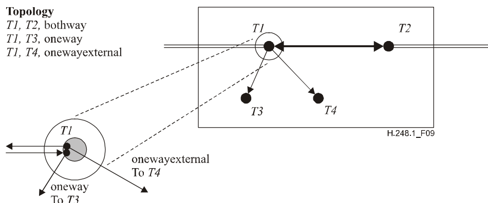
Figure 9/H.248.1 – Onewayexternal contrasted with oneway topology
