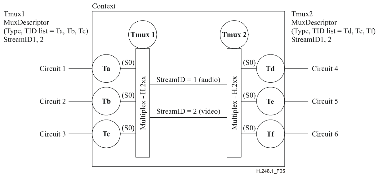
Figure 5/H.248.1 – Multiplexed termination scenario – Circuit-to-circuit
