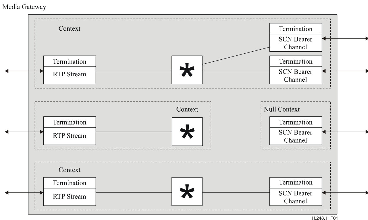
Figure 1/H.248.1 – Example of H.248.1 connection model
