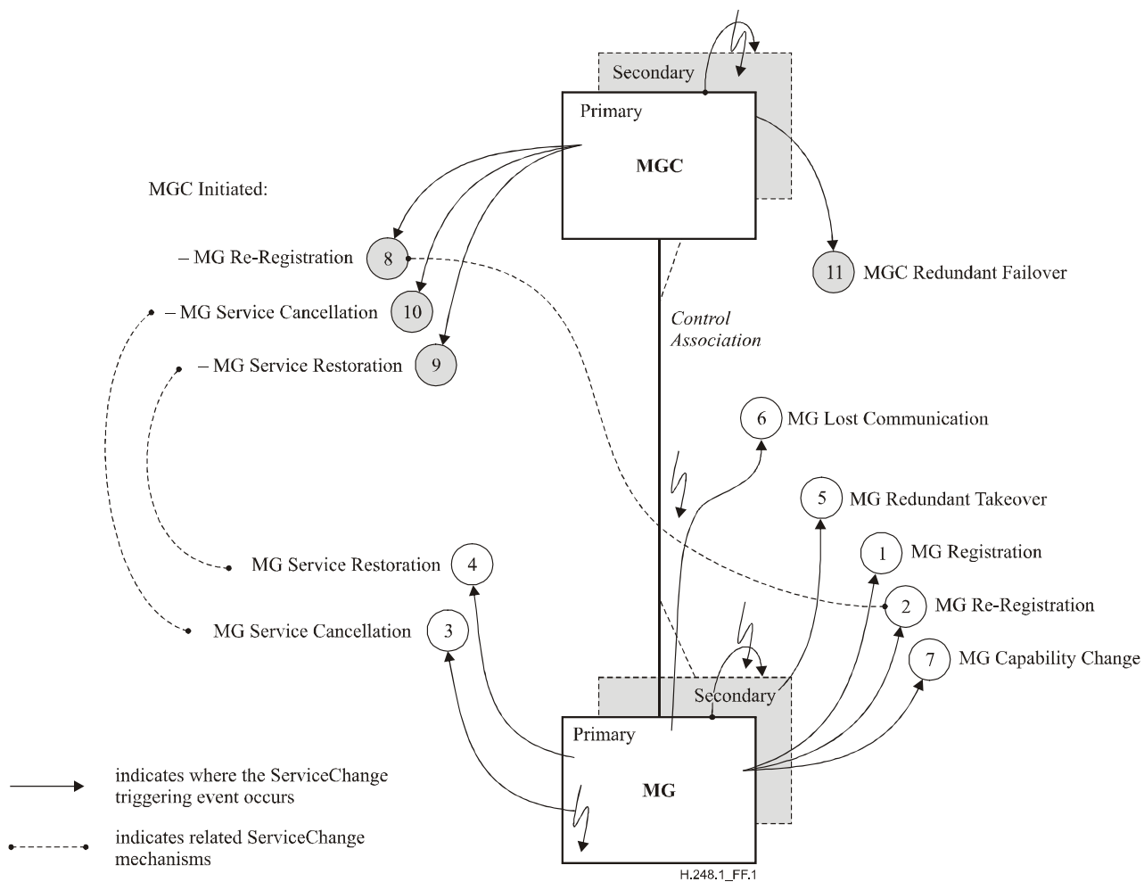
Figure F.1/H.248.1 – Trigger events for ServiceChange
