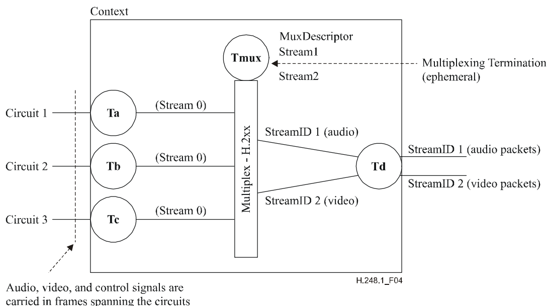
Figure 4/H.248.1 – Multiplexed termination scenario – Circuit-to-packet
