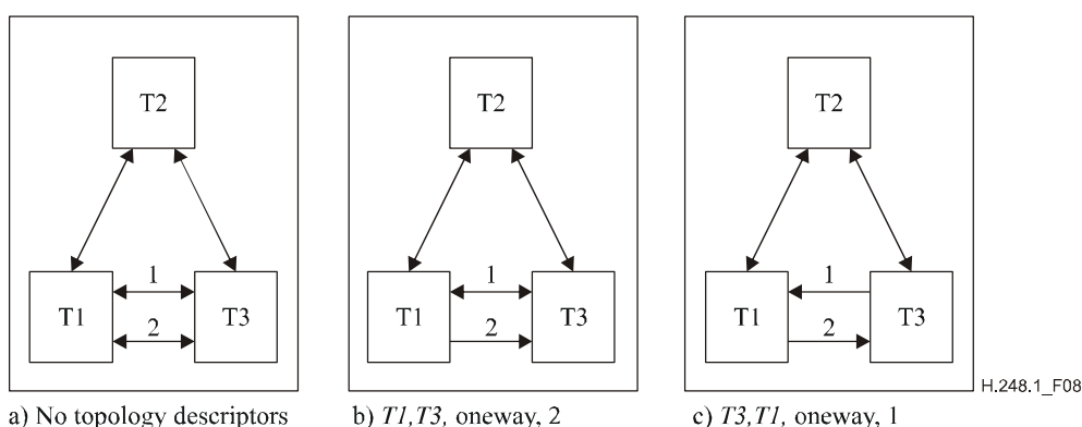
Figure 8/H.248.1 – Example topology at stream level
