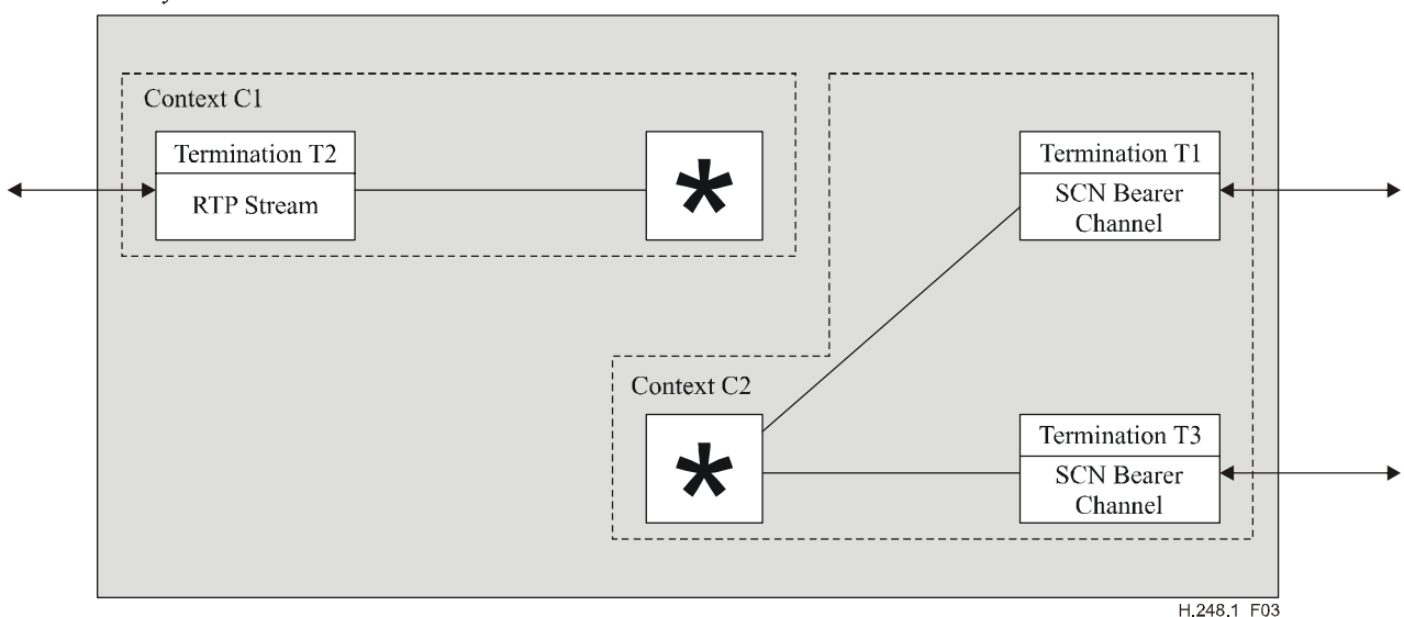
Figure 3/H.248.1 – Example call waiting scenario/answer by T1
