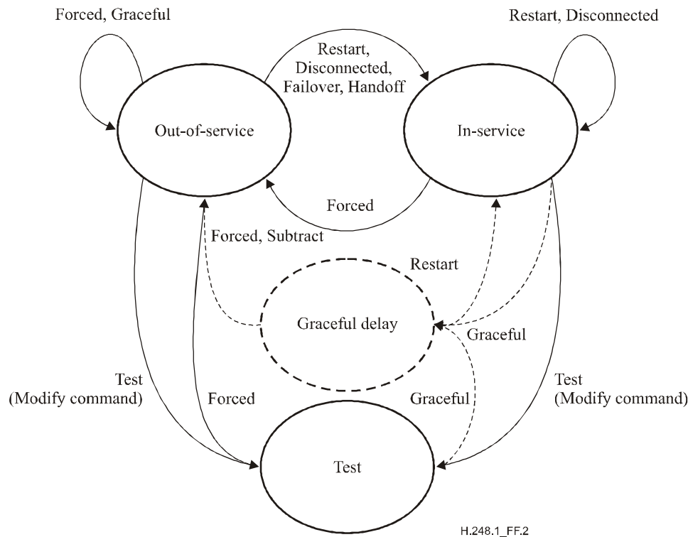
Figure F.2/H.248.1 – Simple ServiceChange state model
