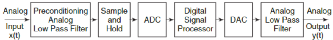
Figure 1.17 Example of a digital signal processing system.
