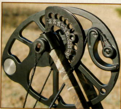
The 2CPW Two-Cam System on the Mission Menace features easy-adjust pivoting draw-length modules. Note the beefy module-locking screw. That screw won't strip out no matter how many times this bow is adjusted.
