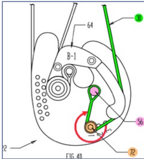
Darlington (Ex. 1004, Fig. 4D)
