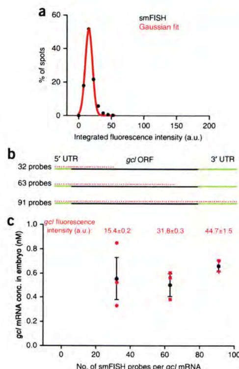
Figure 4 | Determining the fluorescence intensity of a single mRNA molecule. (a) The integrated fluorescence intensities of all detected spots from Figure 3h are plotted as a histogram (black circles) and fitted to a Gaussian curve (red line). The peak of the Gaussian fit determines the average integrated fluorescence intensity of a single gcl mRNA, here hybridized with 32 singly labeled Quasar 670 probes, which, with given imaging and microscope parameters, was 15.4 \pm 0.2 a.u. ( R^2 = 0.99 ). (b,c) gcl was labeled with 32 ( gcl first third (smFISH probes annealing to the first one third of gcl mRNA) probe mix), 63 ( gcl first third and second third smFISH probe mix) or 91 ( gcl first third, second third and third smFISH probe mix) Quasar 670 smFISH probes (b). (c) An average integrated fluorescence intensity of a single gcl mRNA determined ventrally in the early embryo for each probe mix, as described above, and the concentration of gcl mRNA detected for each smFISH probe mix. For each probe mix, an average of three embryos \pm s.e.m. is shown. Red circles, squares and triangles represent individual measurements performed on embryos stained with 32, 63 and 91 gcl smFISH probes, respectively.
