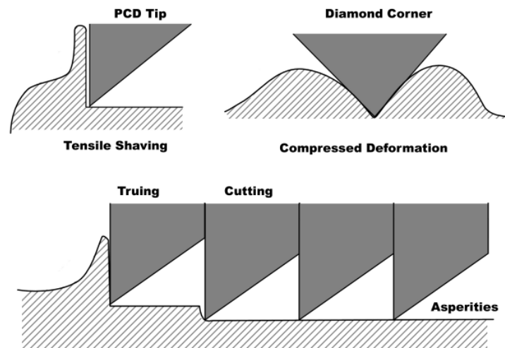
Figure 11. The shaving by tension versus the deforming by compression (top diagram). The blade train that can true the pad before grooving (lower diagram).
