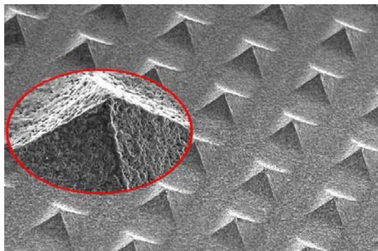
Figure 1. The ADD cutting tips bonded monolithically in PCD matrix material.
