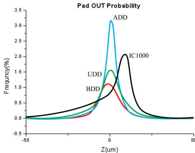
Figure 10. The pad asperities distributions after dressing with ADD, BDD and UDD. Note that the unused pad (IC 1000) was fully leveled on the tips of asperities due the slicing by a sharp steel knife. ADD has the best leveled tips after the pad was dressed with more working crystals. Both UDD & BDD had fewer working crystals so the dressed pad had uneven heights of asperities. In general, the leveling of asperity tips allows uniform and consistent polishing of wafers.
