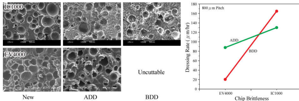
Figure 6. BDD can dress brittle pad materials that may scratch wafer surface. However, ADD can dress resilient polymers to ensure soft landing of delicate IC during CMP.
