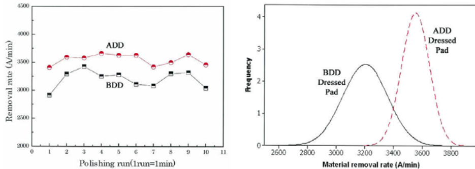
Figure 4. The PCD cutters dressed pad could polish wafer faster with more uniform loading than diamond grits.
