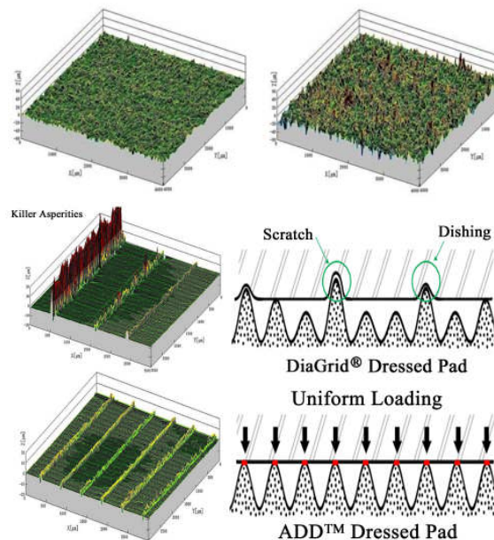
Figure 3. The uniform pad dressing of ADD can avoid the formation of killer asperities that may destruct delicate IC wafers. In the above legend, DiaGrid® refers to BDD pad conditioner.
