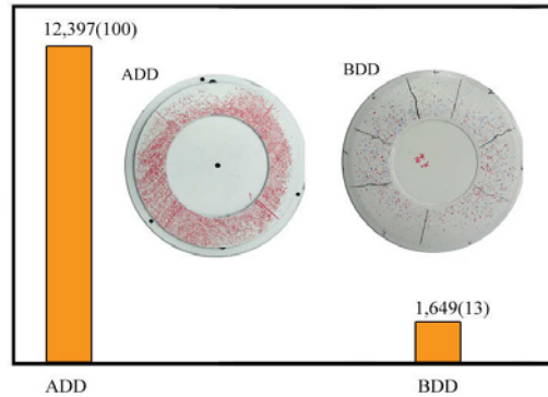
Figure 2. The comparison of working crystals (darkened dots) between ADD and BDD after dressing the pad (IC1000). Both disks have about the same number of cutting tips to begin with the test.
