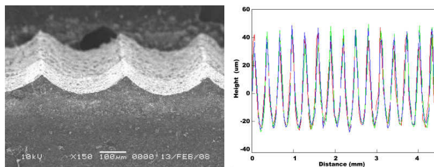
Figure 7. The PCD blade with cutting teeth that can be fully leveled. Note that the cutter tips are leveled within a few microns compared to conventional range of 50 to 100 microns for highest points of discrete diamond grits.
