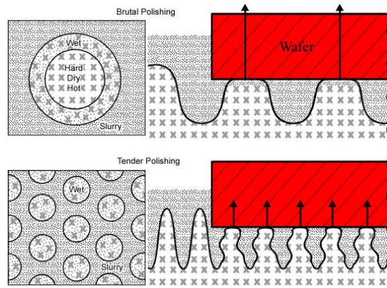
Figure 5. The contrast between brutal polishing with BDD dressed pad and tender polishing with ADD dressed pad.
