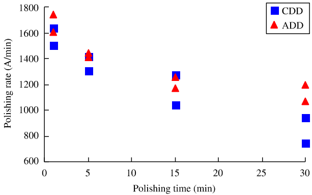
Fig. 12. Variation in polishing rate with polishing time.
